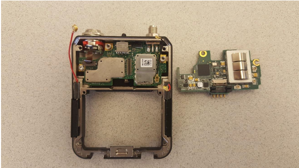
ADX1 Internal View – Rear
