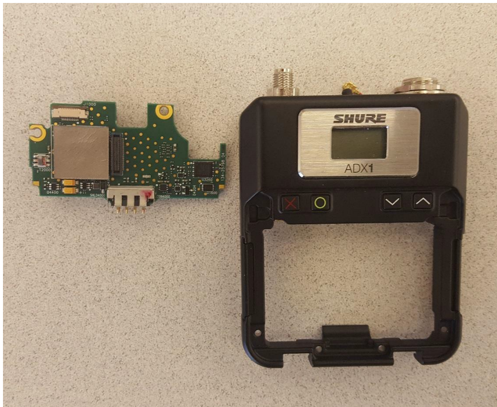
ADX1 Internal View -- Front
