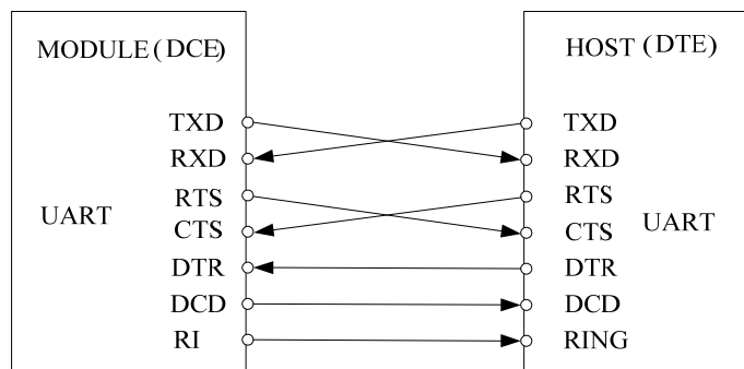
Figure 12: UART full modem
