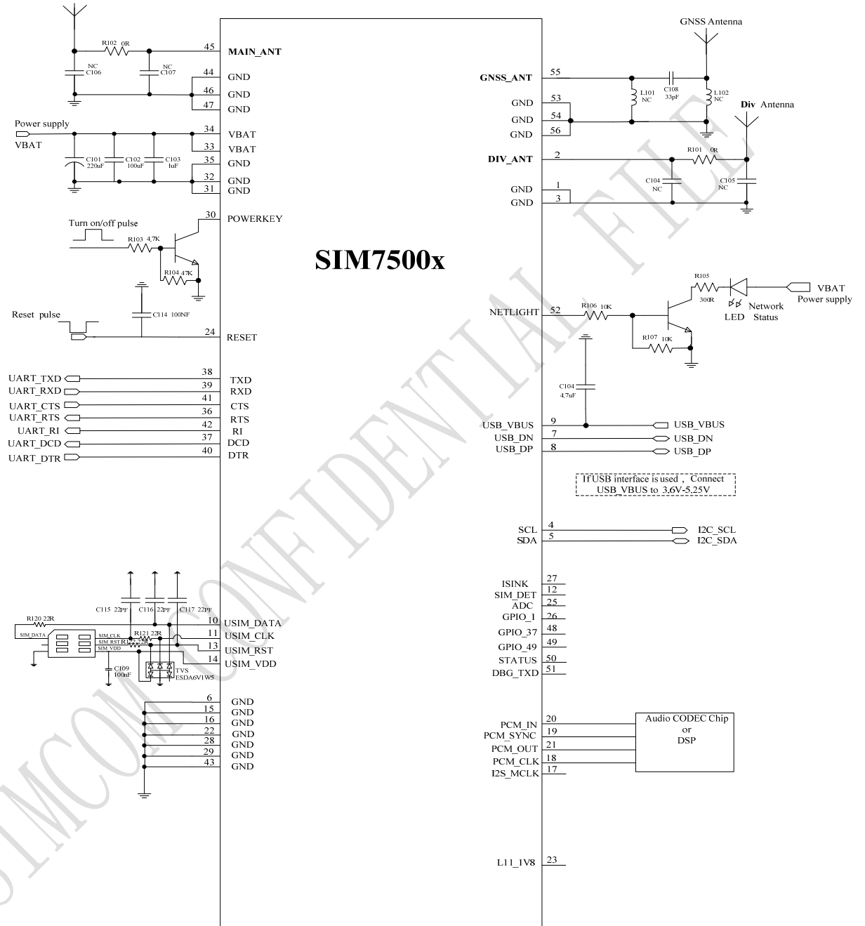
Figure 38: Reference design
