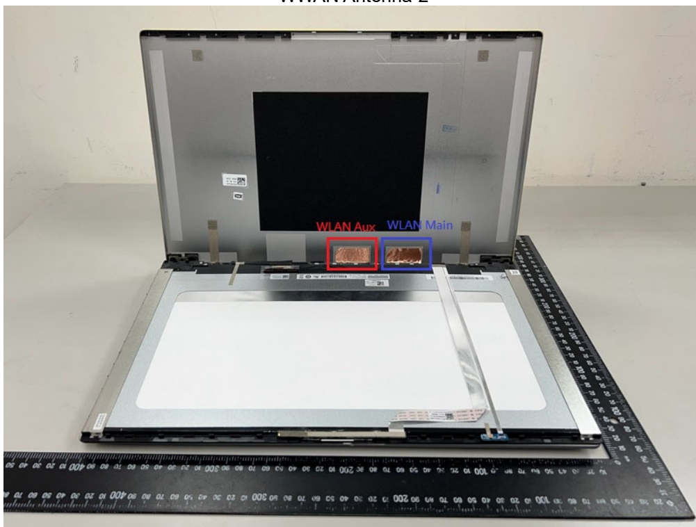
WWAN Antenna-2
