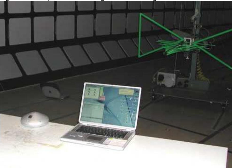
Figure 5.3: front picture of test configuration, for testing above 1 GHz.
