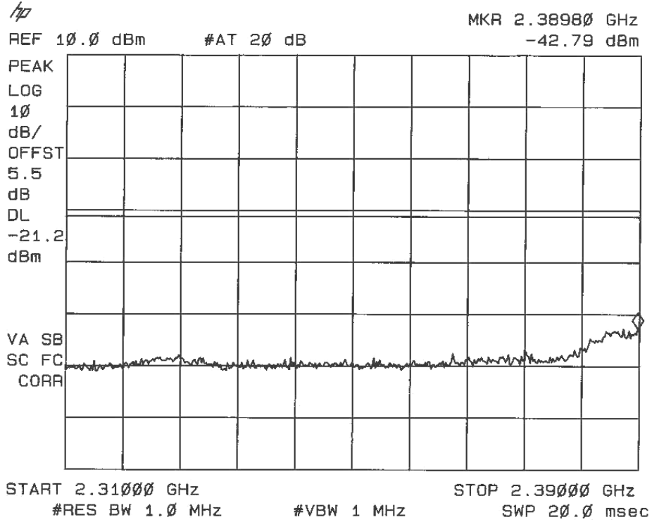
Figure 9.2: peak values in restricted band, All bitrate settings, conducted measurement, corrected for 2 dBi antenna gain and 2.6 dB cable losses. 74 dB \mu V/m :: -21.2 dBm display line setting.
