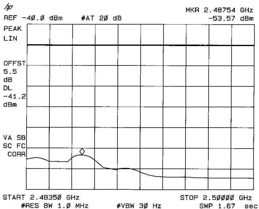
Figure 9.3: average values in restricted band, All bitrate settings, conducted measurement, corrected for 2 dBi antenna gain and 2.6 dB cable losses. 54 dB \mu V/m :: -41.2 dBm display line setting.
