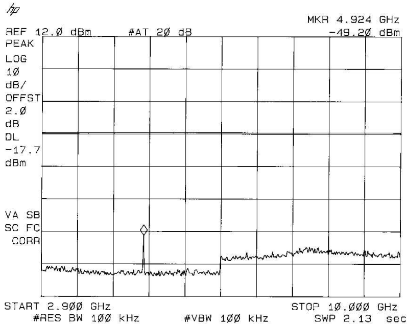
Figure 9.10: conducted emission outside restricted band. Display line :: -20 dB limit line. Corrected (offset) for cable losses.
