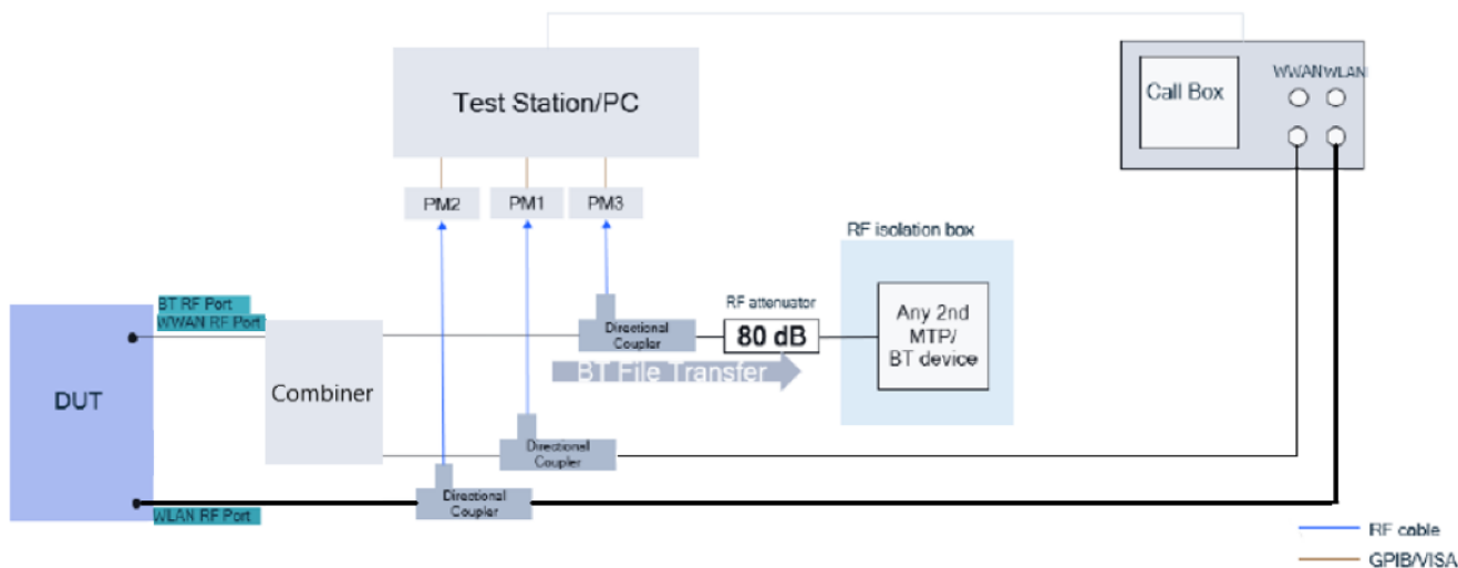
(g) Appendix A – Test Setup Photo 10
