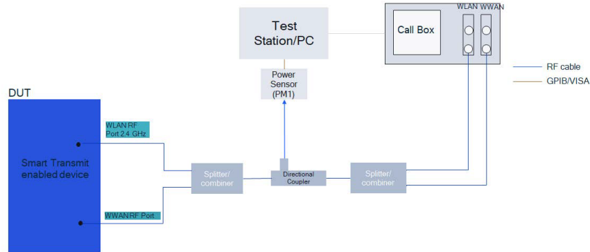
(f) Appendix A – Test Setup Photo 7
