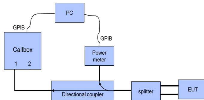
(b) Appendix A – Test Setup Photo 6
