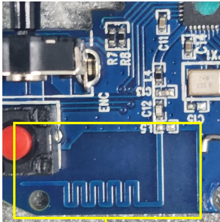
Pattern Antenna
