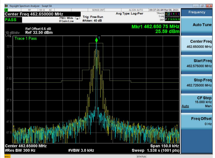
Channel 19: 462.6500MHz
