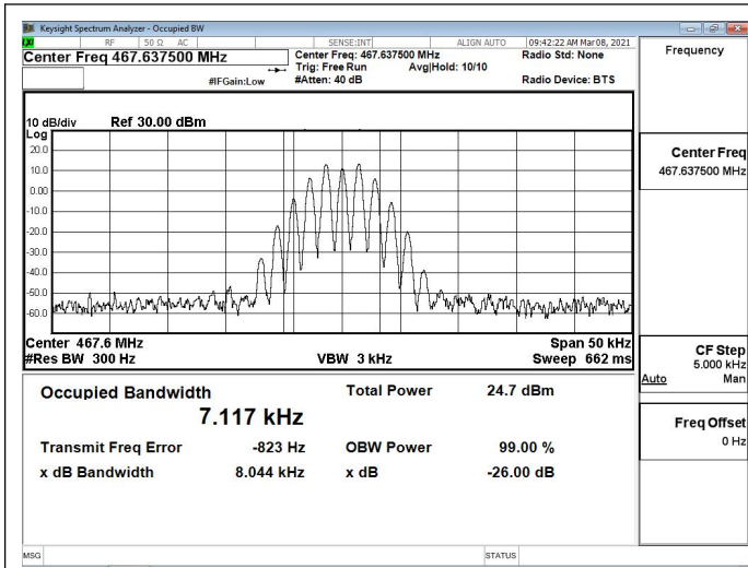
Channel 11: 467.6375MHz
