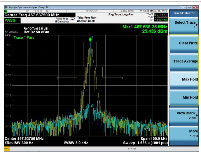
Channel 11: 467.6375MHz
