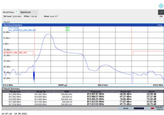
LTE-M Band 26 QPSK 3MHz CH-Low 1RB
