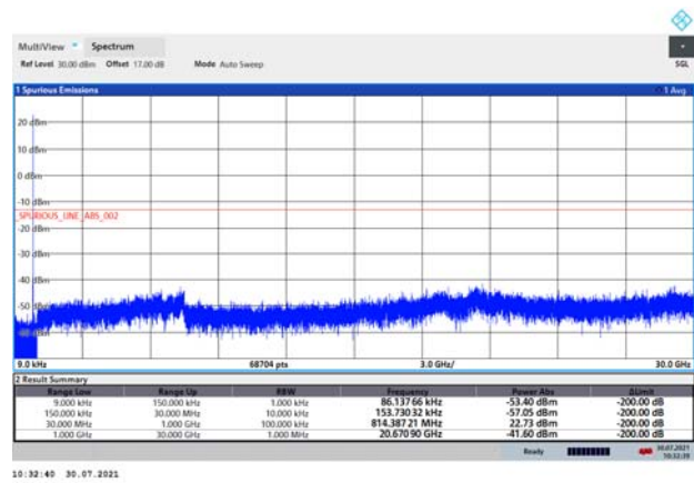
LTE-M Band 26 3MHz CH Middle 9kHz~30GHz
