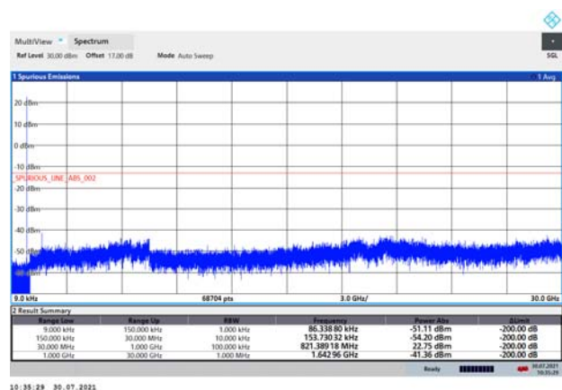
LTE-M Band 26 3MHz CH High 9kHz~30GHz
