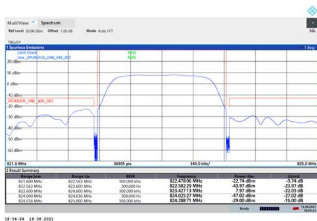
LTE-M Band 26 QPSK 3MHz CH-High 1RB
