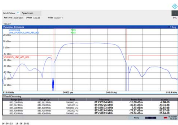
LTE-M Band 26 QPSK 1.4MHz CH-Low 100%RB
