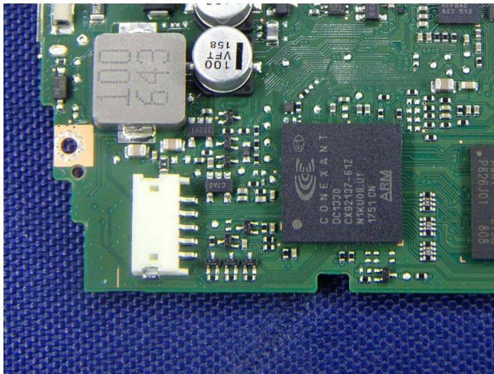
(28) EUT Photo
