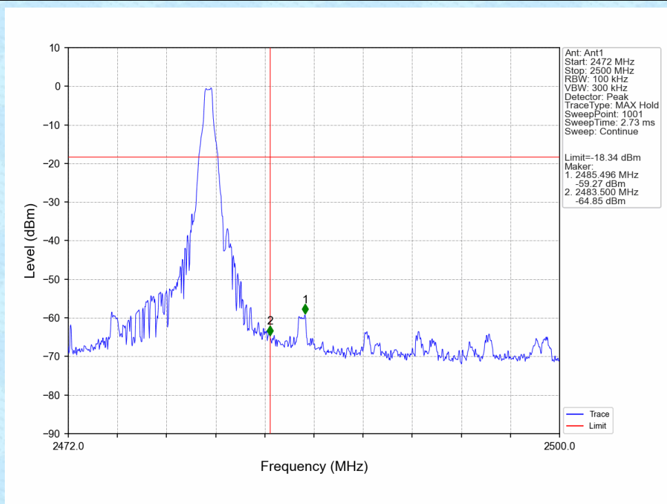
GFSK_DH5_HCH_2480MHz_Ant1_NTNV
