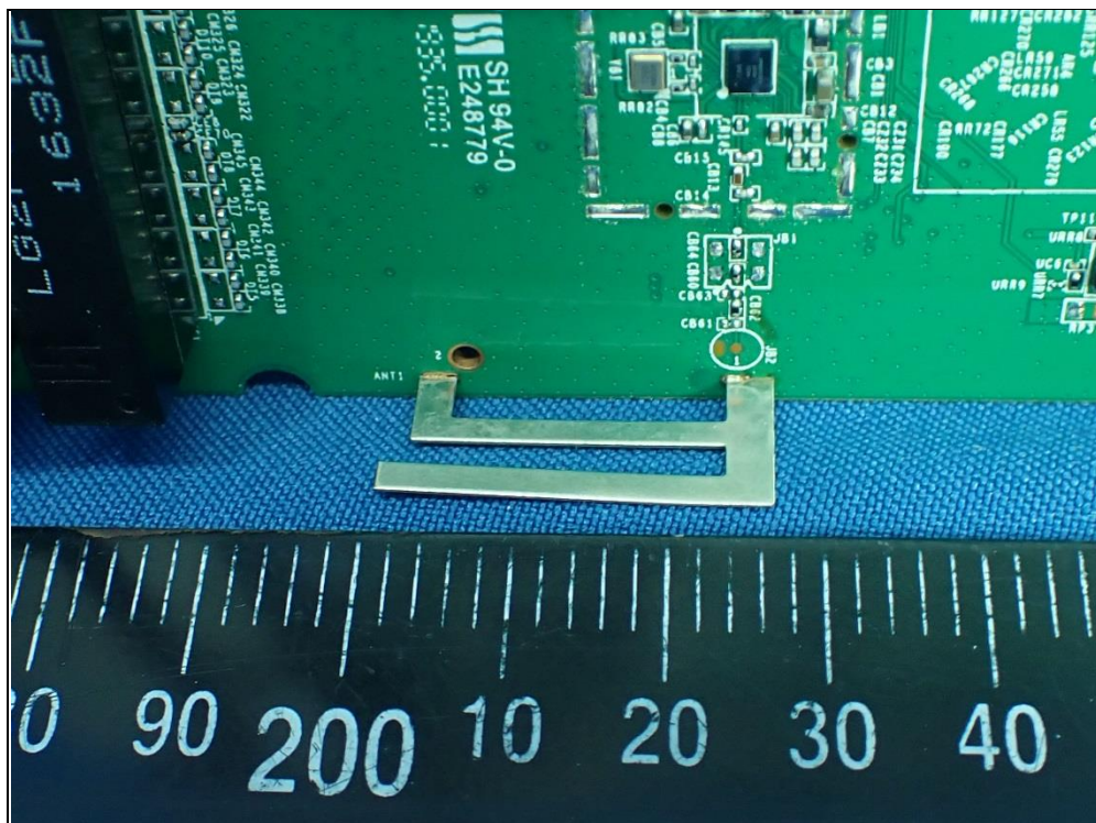
BT Antenna
