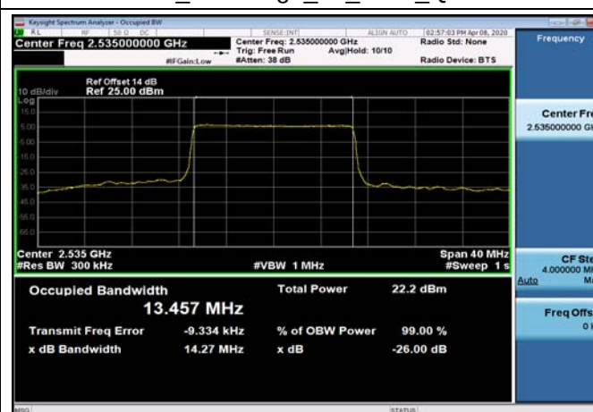
FDD07_MidRange_15_2535_QPSK
