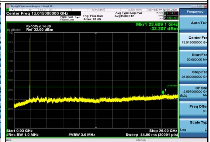
FDD07_HighRange_5MHz_30MHz~26GHz
