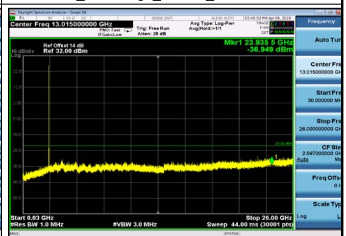
FDD07_LowRange_15MHz_30MHz~26GHz
