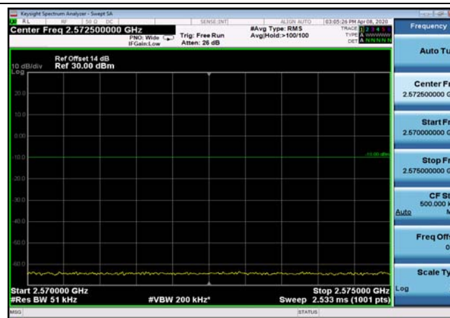
FDD07_10MHz_2505_QPSK_OneRB_high _ExtraBands_Range_2570~2575
