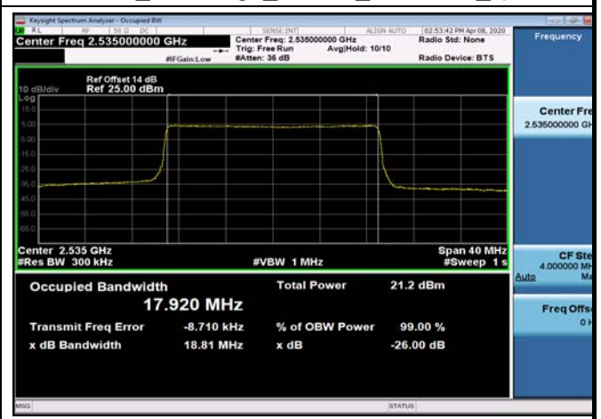
FDD07_MidRange_20MHz_2535MHz_Q16
