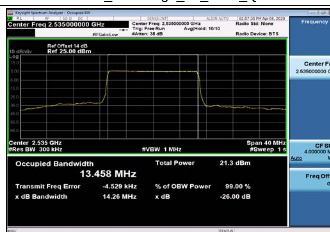
FDD07_MidRange_15_2535_Q16
