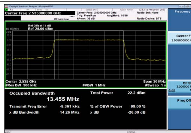
FDD07_MidRange_15MHz_2535MHz_QPSK
