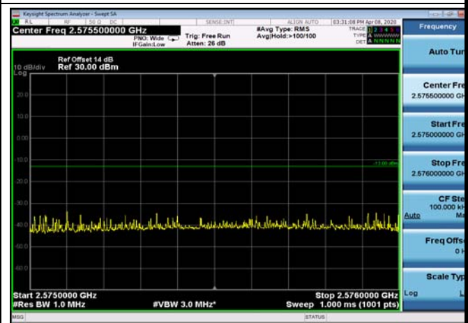
FDD07_15MHz_2562.5_Q16_OneRB_high _ExtraBands_Range_2575~2576
