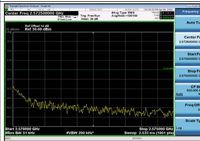
FDD07_15MHz_2562.5_Q16_OneRB_high _ExtraBands_Range_2570~2575
