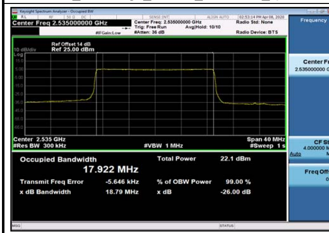
FDD07_MidRange_20MHz_2535MHz_QPSK
