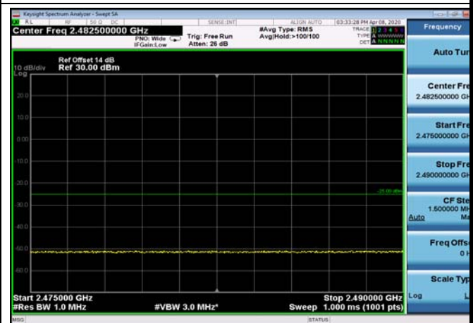
FDD07_15MHz_2562.5_QPSK_fullRB _ExtraBands_Range_2475~2490
