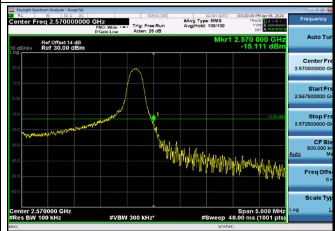
HighRange_FDD07_5MHz_2567.5_OneRB _high_Q16
