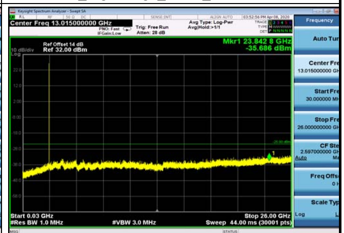
FDD07_LowRange_15MHz_30MHz~26GHz
