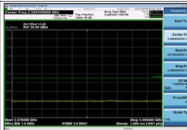
FDD07_20MHz_2510_QPSK_OneRB_high_ExtraBands_Range_2576~2595
