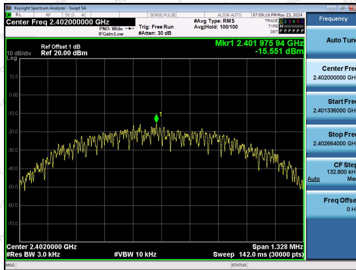
BLE_1M-Ant1-2402-PASS
