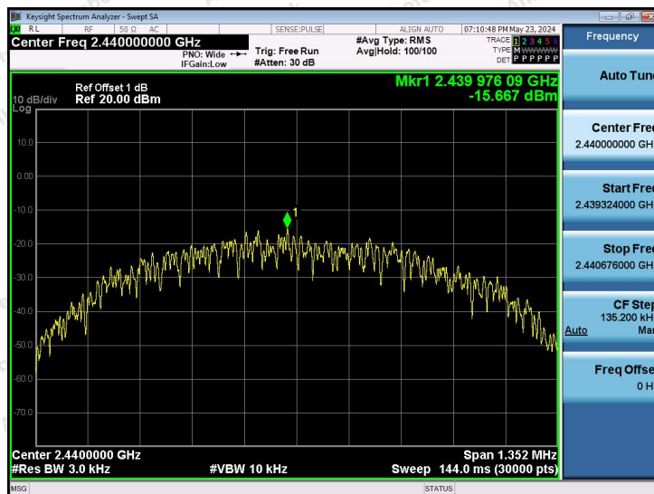
BLE_1M-Ant1-2440-PASS
