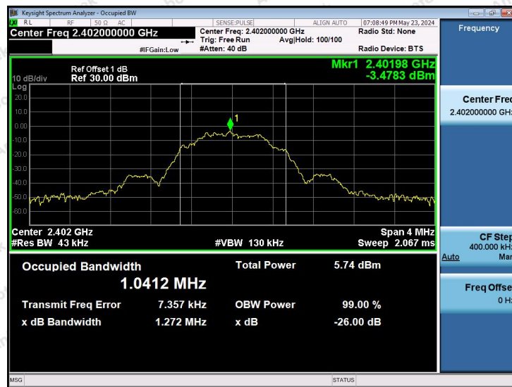
BLE_1M-Ant1-2402
