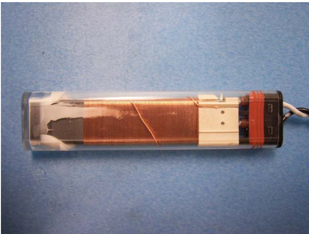
Antenna Bottom
