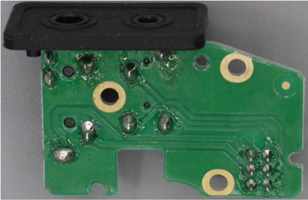
Figure E23.7 – Internal Photo – Accessory PCB Bottom
