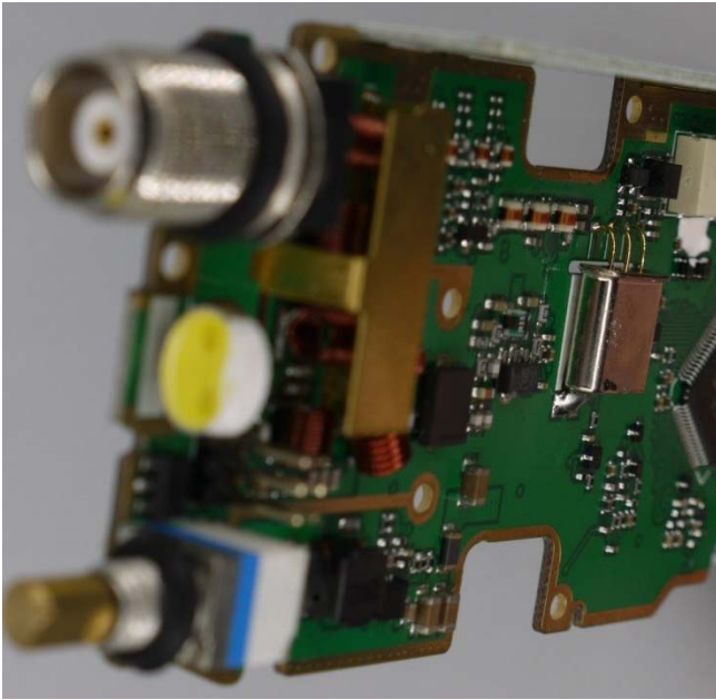
Figure E23.5 – Internal Photo – Main PCB Top End
