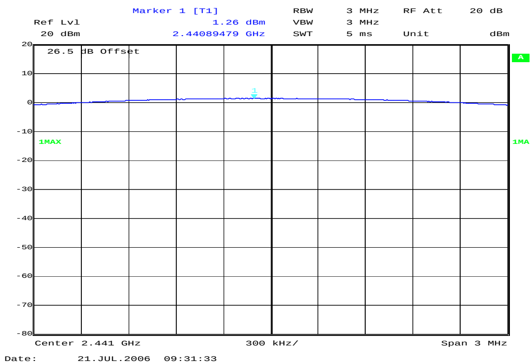
Plot 2: (2441 MHz)
