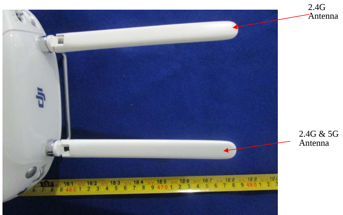
EUT –AntennaView
