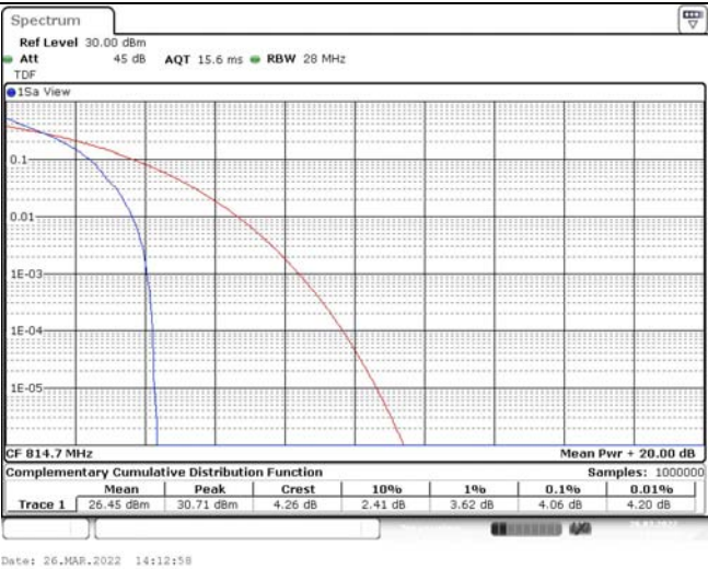
Band26-1.4MHz-QPSK-26697-1RB#0
