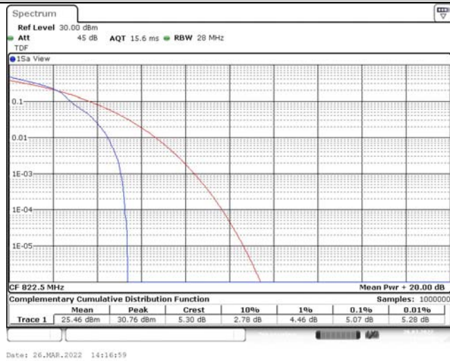
Band26-3MHz-16QAM-26775-1RB#0
