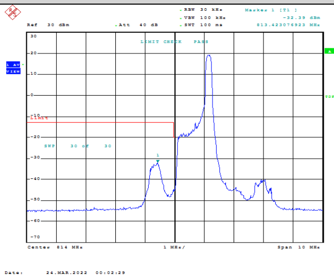
Band26-1.4MHz-QPSK-26697-1RB#5
