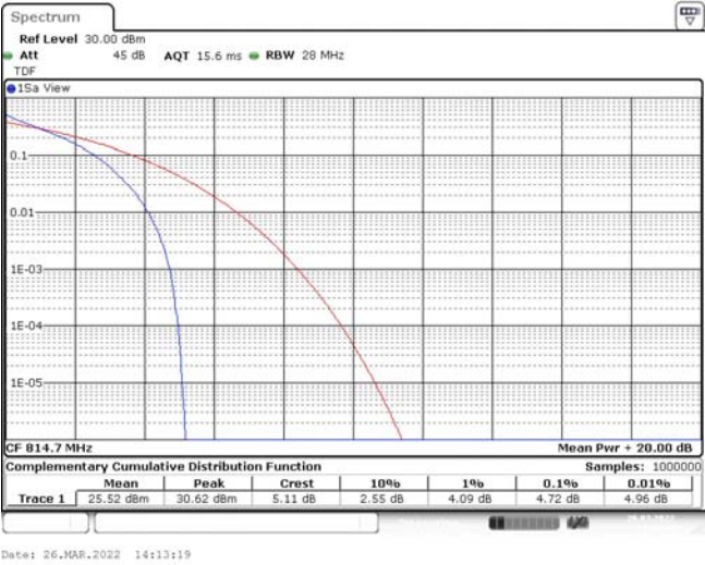
Band26-1.4MHz-QPSK-26697-6RB#0
