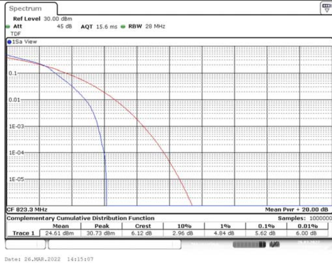
Band26-1.4MHz-16QAM-26783-6RB#0
