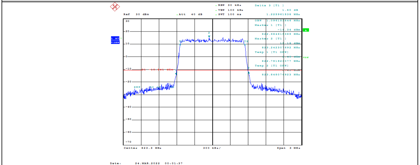
Band26-1.4MHz-QPSK-26783-6RB#0-1.096
