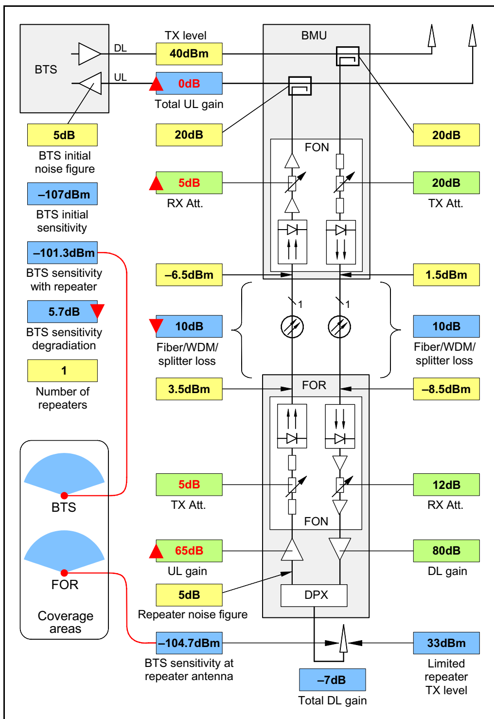
Figure 6-6. One FOR, low optical loss, high uplink gain and attenuation
