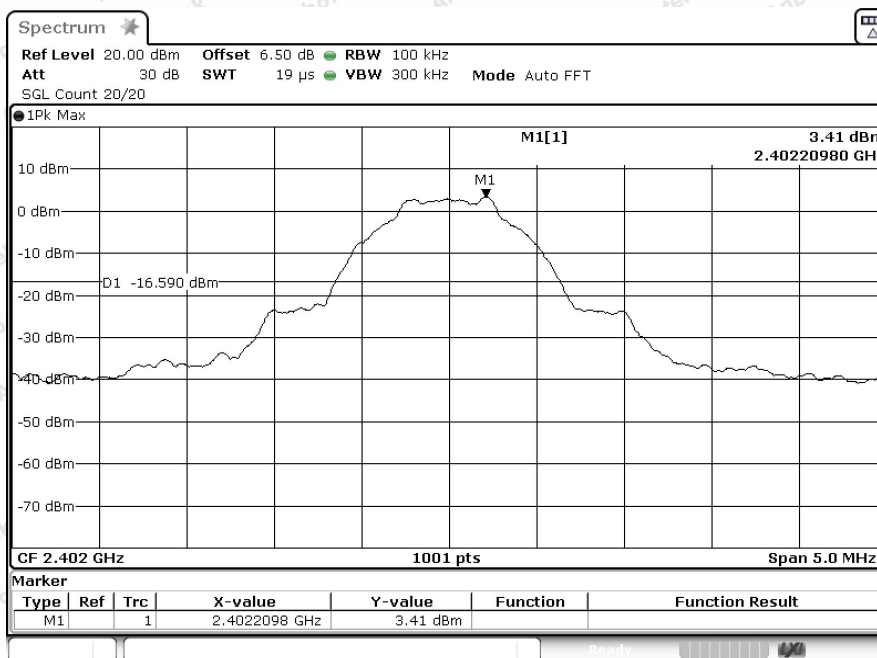
1_Reference_Level_NVNT_ANT1_1Mbps_2402
