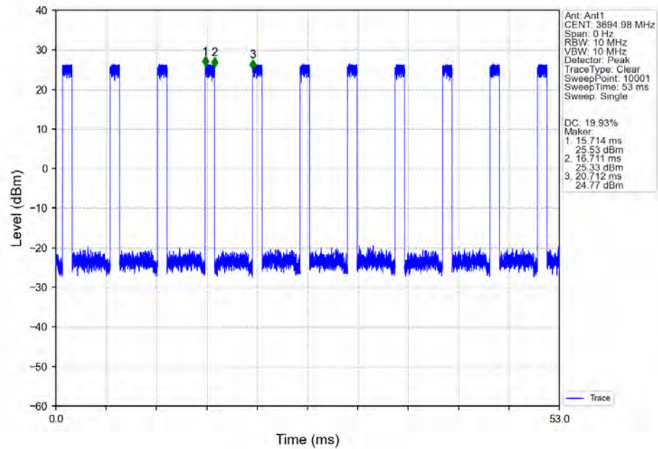
n48_30kHz_SISO_NTNV_10MHz_CP-OFDM_16_QAM_3694.98MHz_Inner_Full_Ant1
