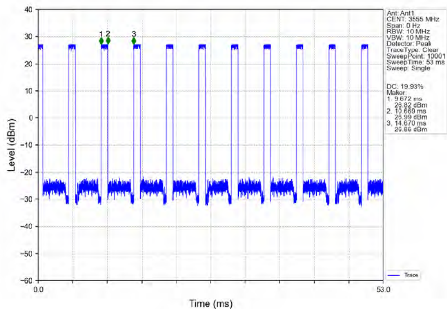
n48_30kHz_SISO_NTNV_10MHz_DFT-s-OFDM_16_QAM_3555MHz_Inner_Full_Ant1
