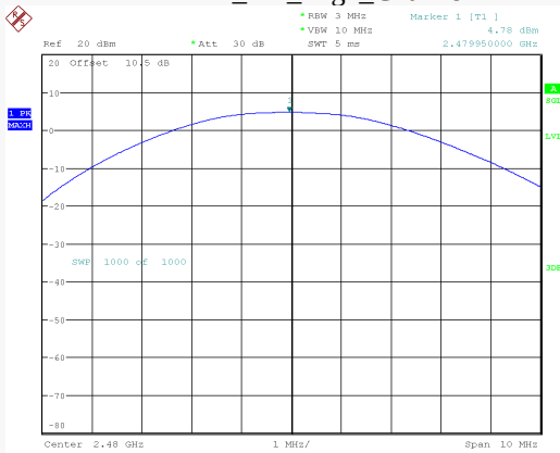
BLE_2M_High_Channel
