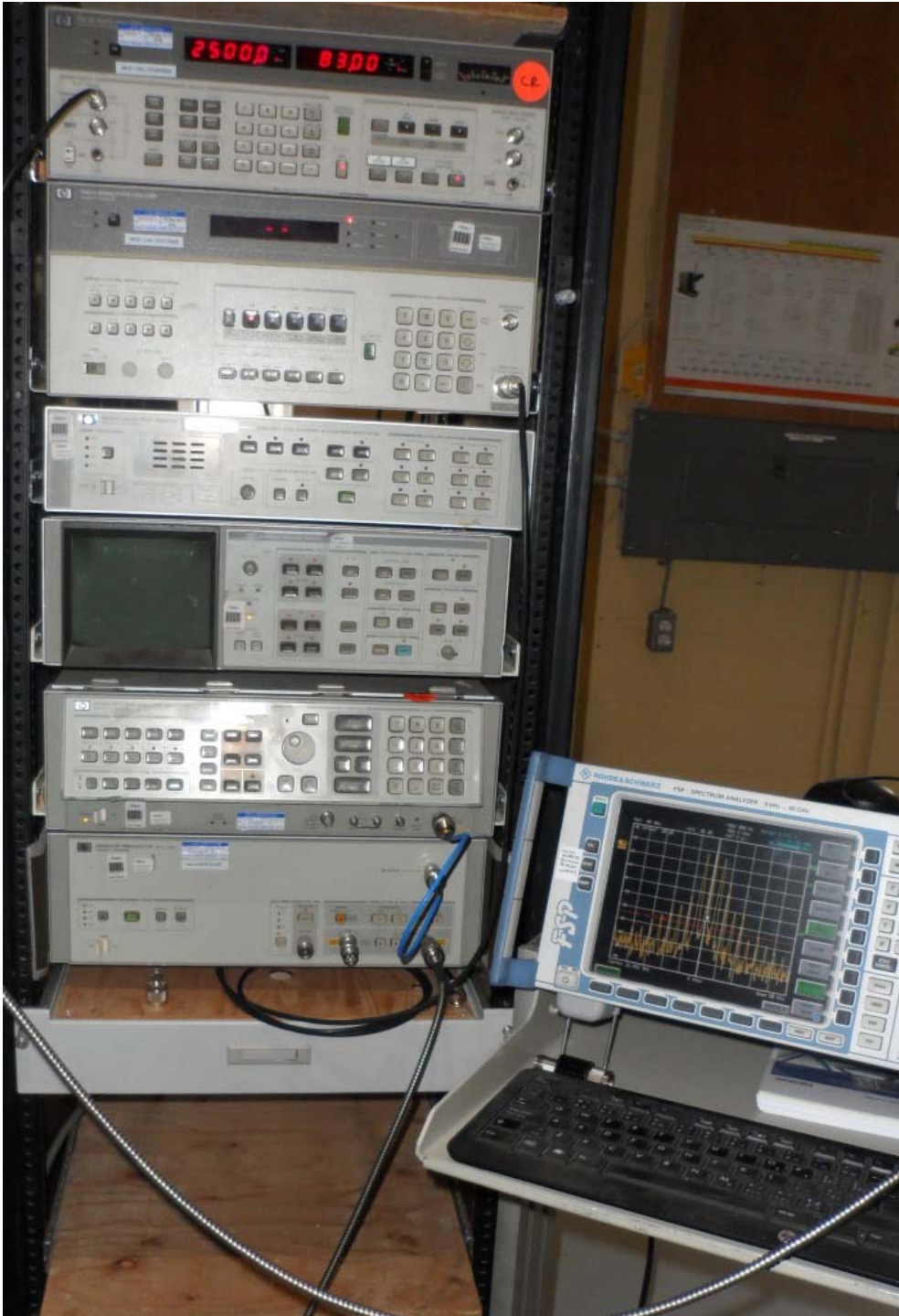
Figure E21.3 – Setup Photo – Occupied Bandwidth
