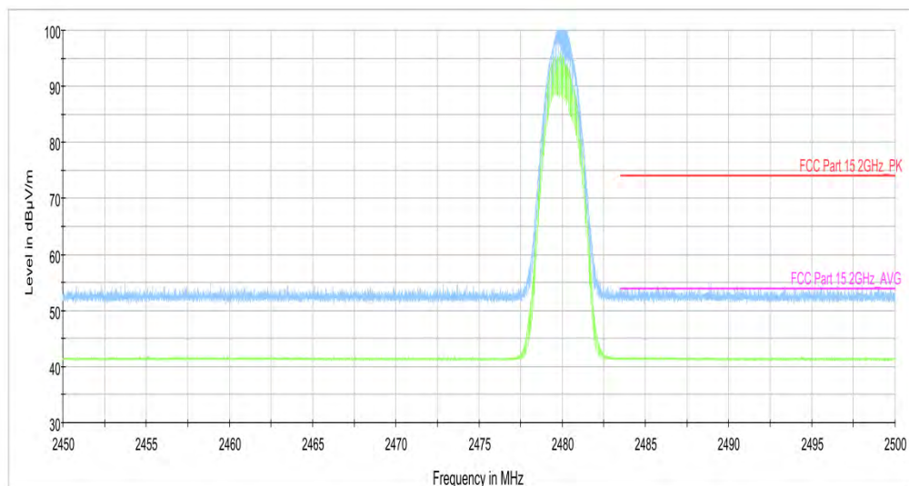
Fig.18. Frequency Band Edges: 8DPSK, Channel 78, 2.45 GHz - 2.50GHz
