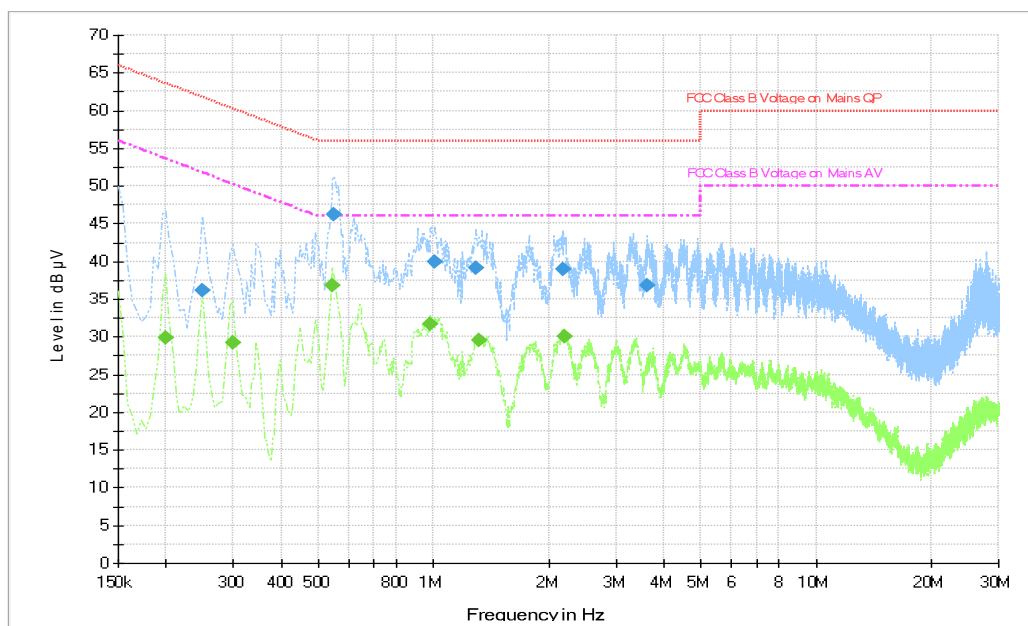
Fig.B.11.2 AC Powerline Conducted Emission-Idle
