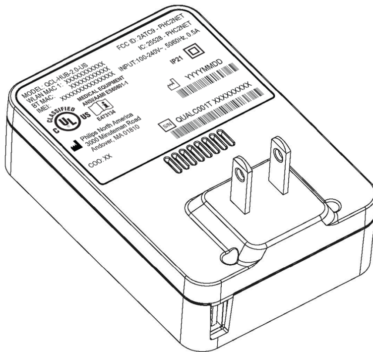
Figure 3: 2net2 LTE Hub FCC/IC label placement
