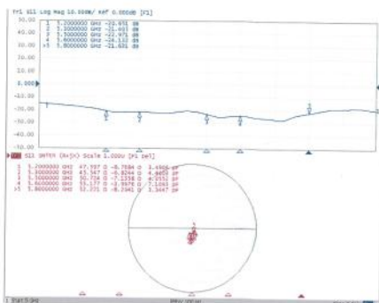
Impedance Measurement Plot for Head TSL
