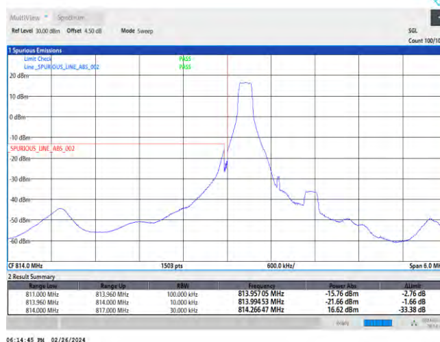
Band26-1.4MHz-QPSK-26697-6RB#0
