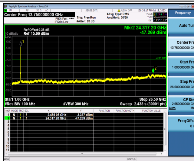
11N40SISO_Ant1_2452_1000-26500
