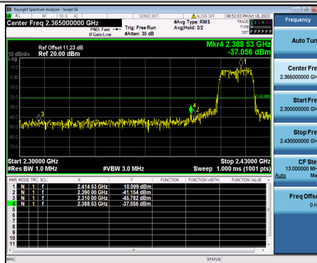
11G_Ant1_Low_2412_Peak
