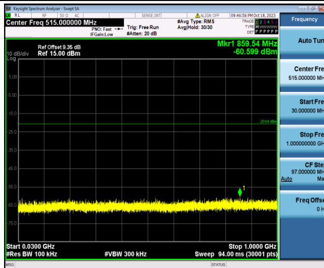
11N20SISO_Ant1_2437_30-1000
