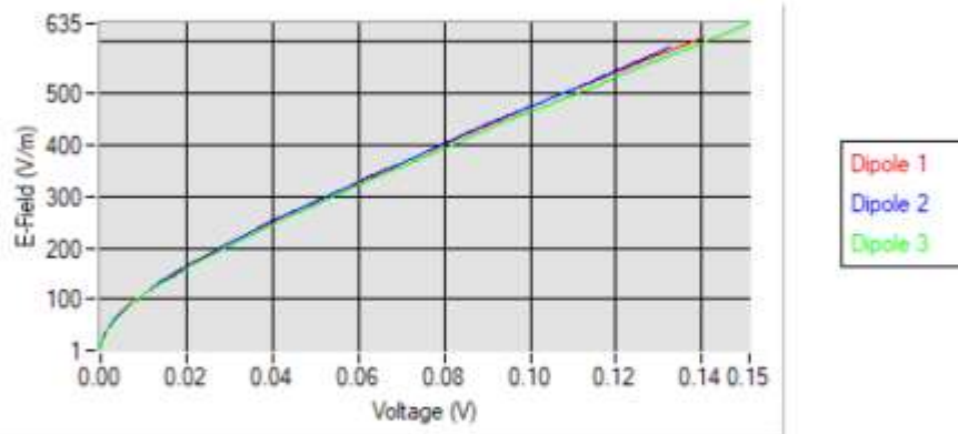
Calibration curves
