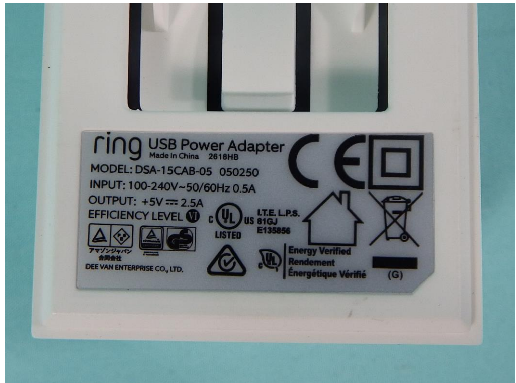
Outdoor Adapter
