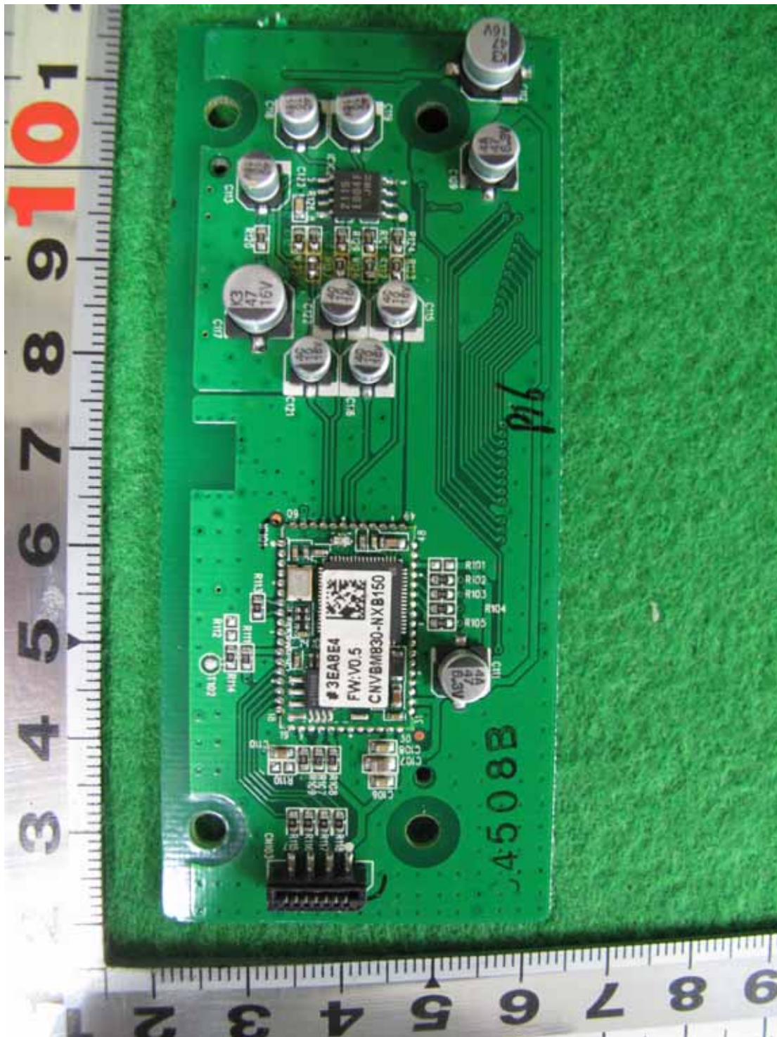
Front Side View of RF board
