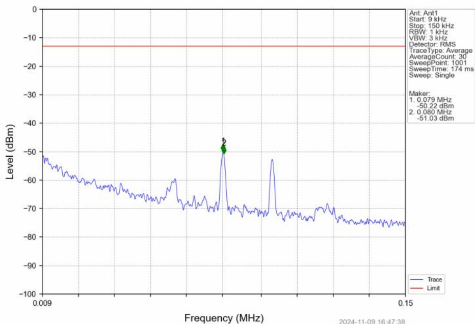
Band66 10MHz QPSK LCH 1715MHz RB 1 0 NTN
