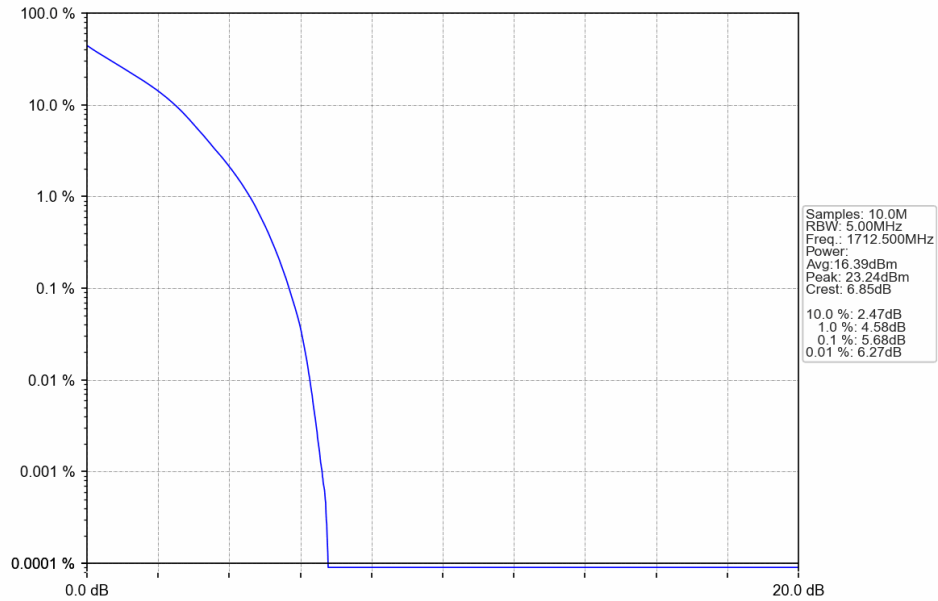
Band4_5MHz_QPSK_LCH_1712.5MHz_RB_25_0_NTNV
