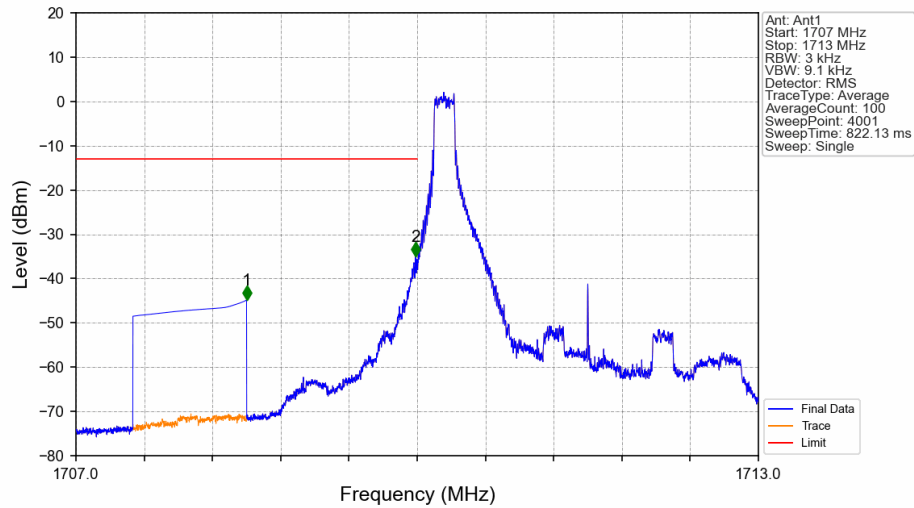
Band4_3MHz_QPSK_LCH_1711.5MHz_RB_1_0_NTNV
