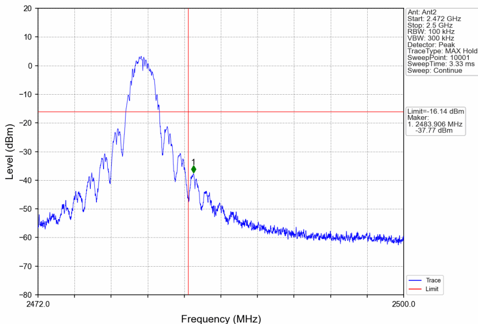
Zigbee_HCH_2480MHz_Ant2_NTNV
