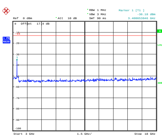
eMTC Band 4 1.4MHz CH-Low 3GHz~18GHz
