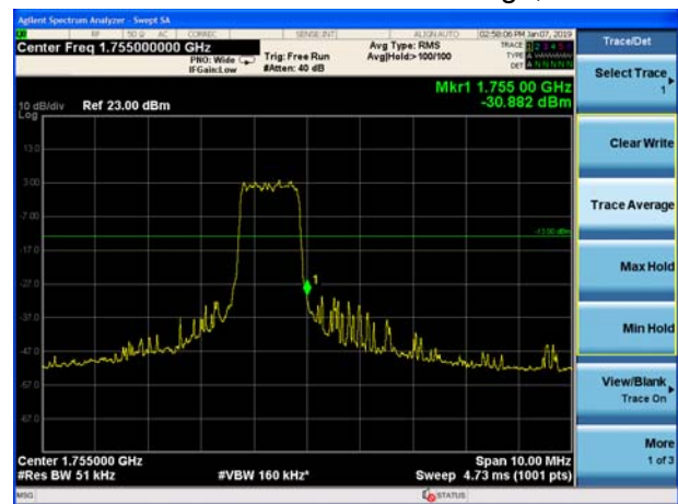
eMTC Band 4 QPSK 3MHz CH-High, 1 RB
