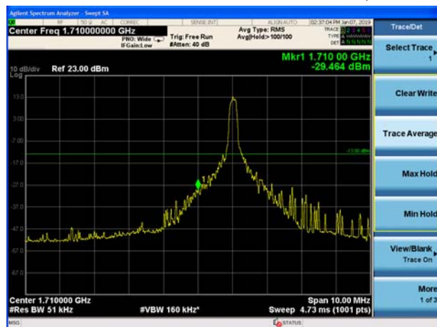
eMTC Band 4 16QAM 15MHz CH-Low, 1 RB
