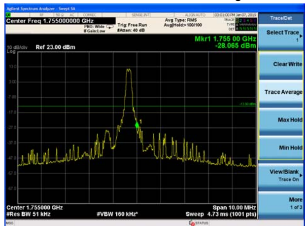
eMTC Band 4 16QAM 5MHz CH-High, 100%RB
