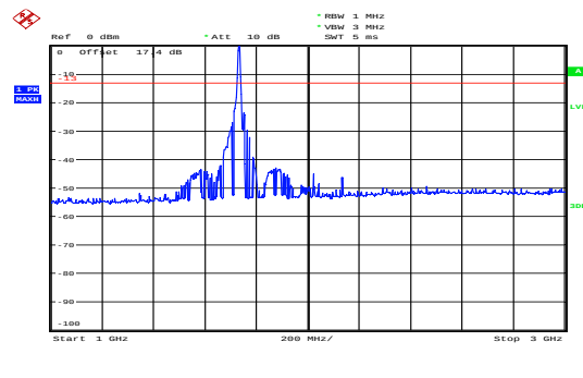
eMTC Band 4 1.4MHz CH-Middle 1GHz~3GHz
