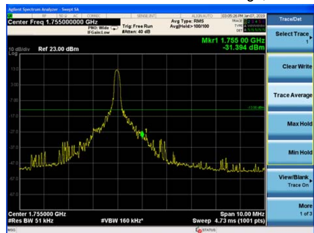
eMTC Band 4 16QAM 15MHz CH-High, 1 RB
