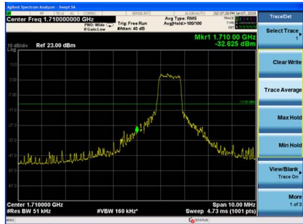
eMTC Band 4 16QAM 20MHz CH-Low, 1 RB
