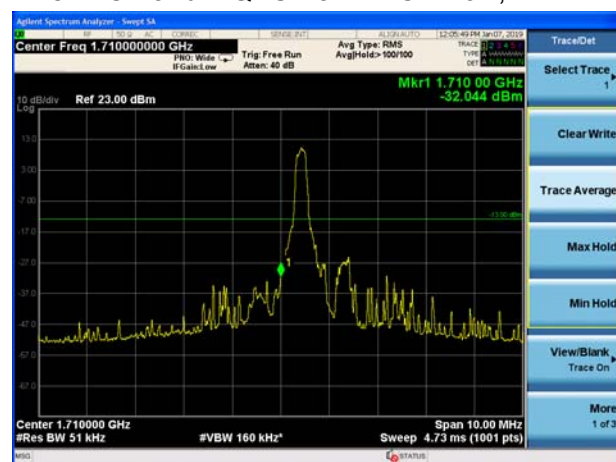
eMTC Band 4 QPSK 3MHz CH-Low, 1 RB
