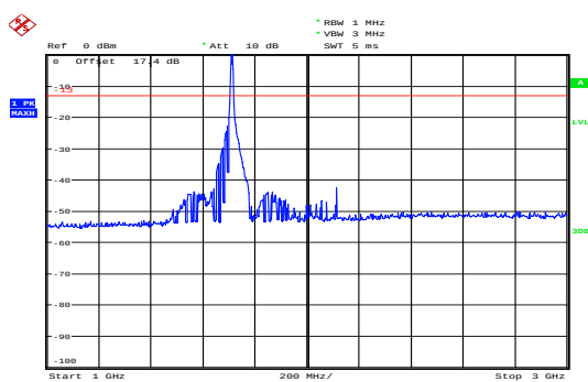
eMTC Band 4 1.4MHz CH-Low 1GHz~3GHz
