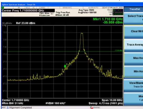
eMTC Band 4 QPSK 20MHz CH-Low, 100%RB
