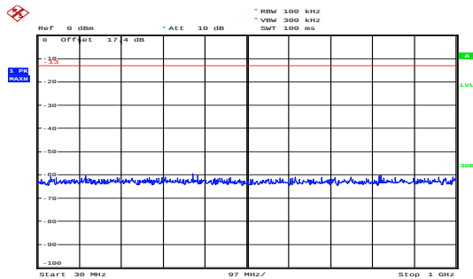
eMTC Band 4 1.4MHz CH-Low 30MHz~1GHz
