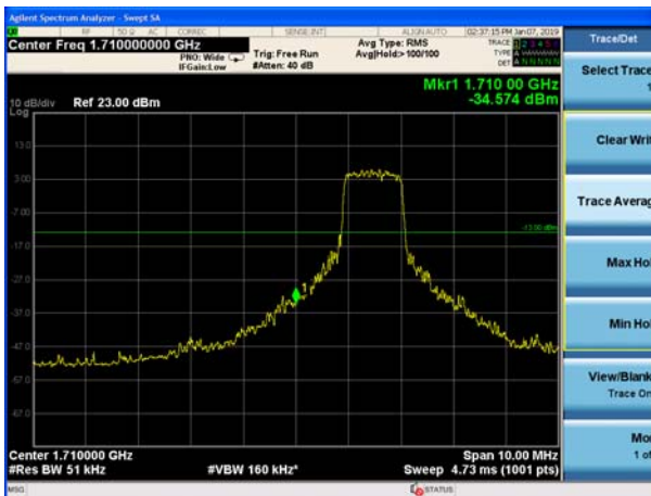
eMTC Band 4 QPSK 20MHz CH-Low, 1 RB
