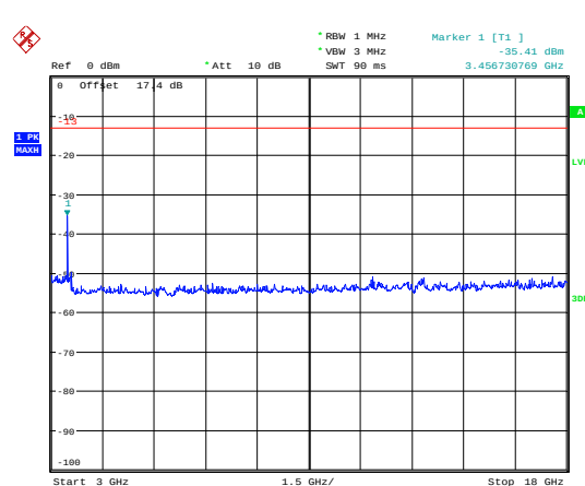
eMTC Band 4 1.4MHz CH-Middle 3GHz~18GHz
