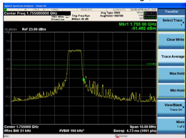
eMTC Band 4 16QAM 3MHz CH-High, 1 RB
