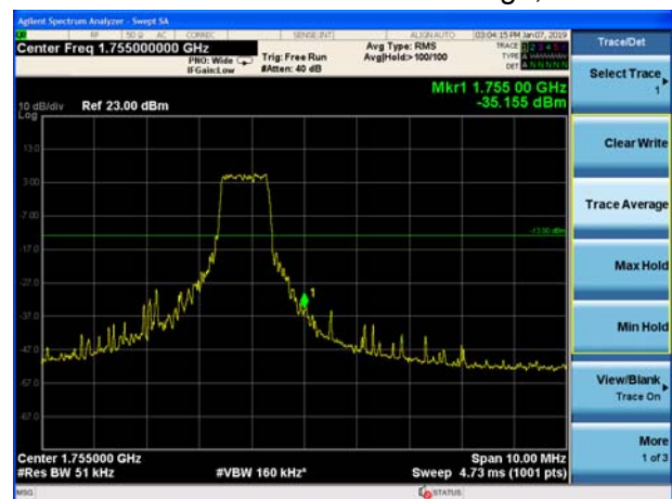
eMTC Band 4 16QAM 15MHz CH-High, 1 RB
