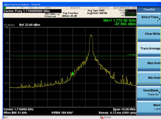
eMTC Band 4 16QAM 20MHz CH-Low, 100%RB
