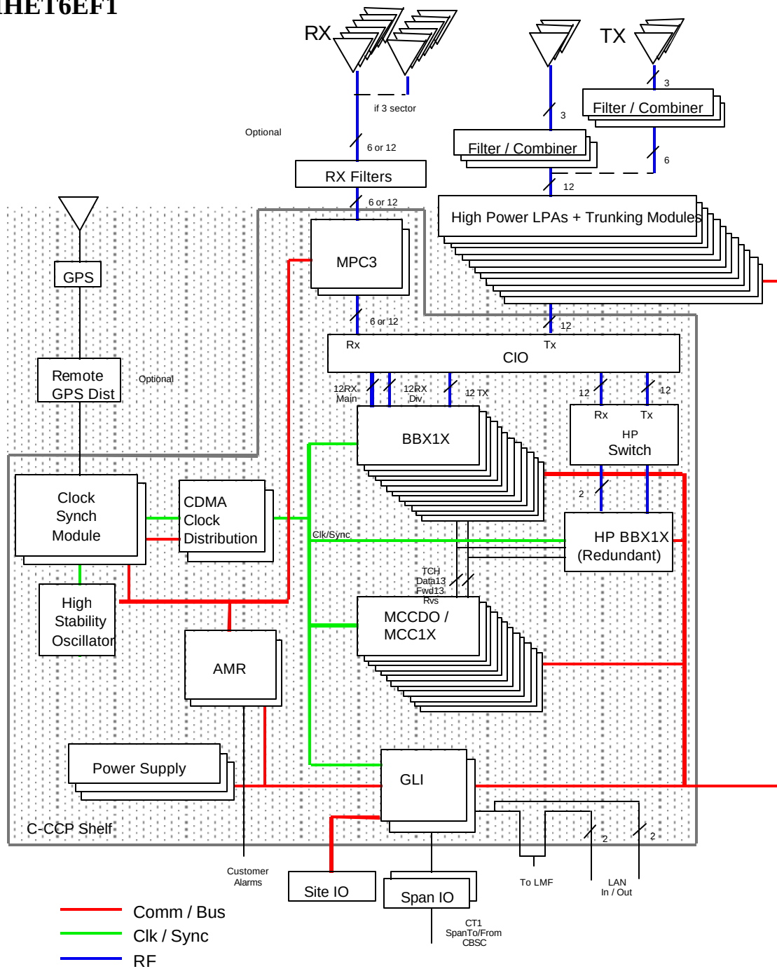
SC4812T 1X / 1X-EVDO @ 1.9 GHz CDMA BTS Frame Block Diagram
