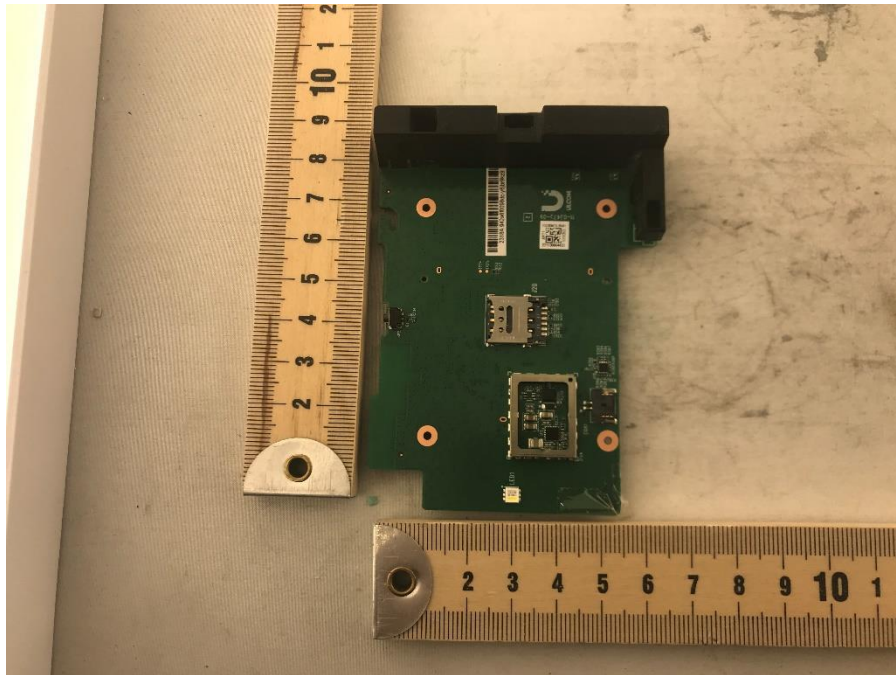
Photograph 6: Top Side Of PCB With Can Off
