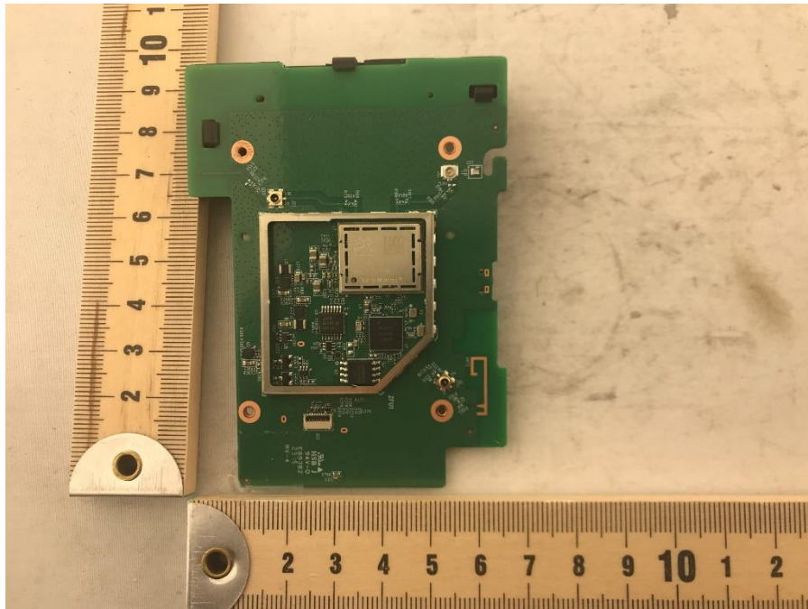
Photograph 7: Bottom PCB With Can Off
