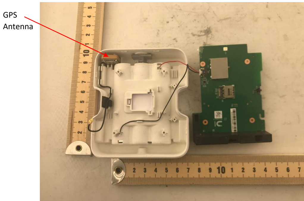
Photograph 4: Internal View of DUT With PCB Out of Case
