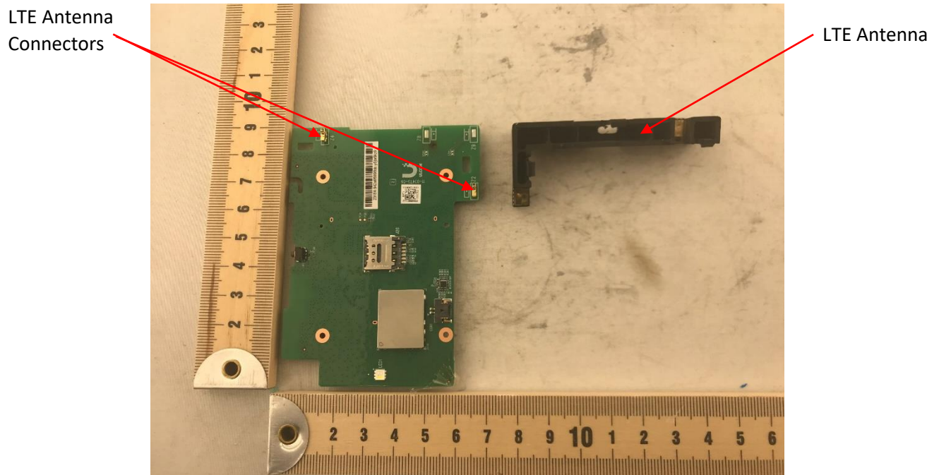
Photograph 8: Top PCB With LTE Antenna Removed
