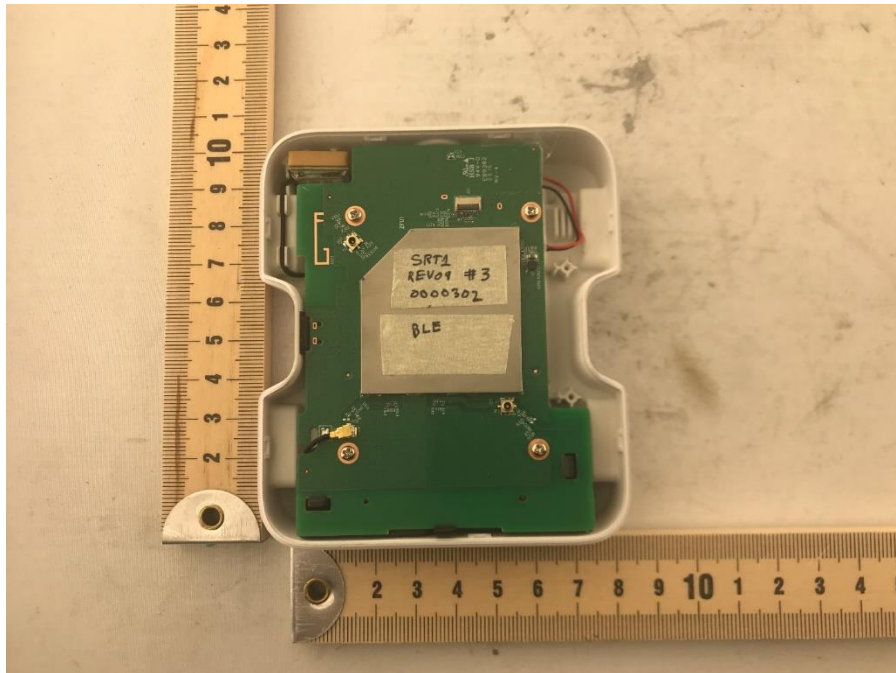
Photograph 2: Internal View of DUT With Back Cover Off
