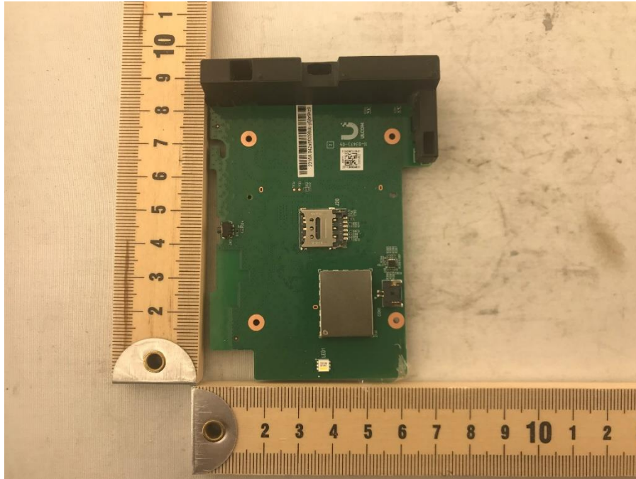
Photograph 5: Top Side Of PCB
