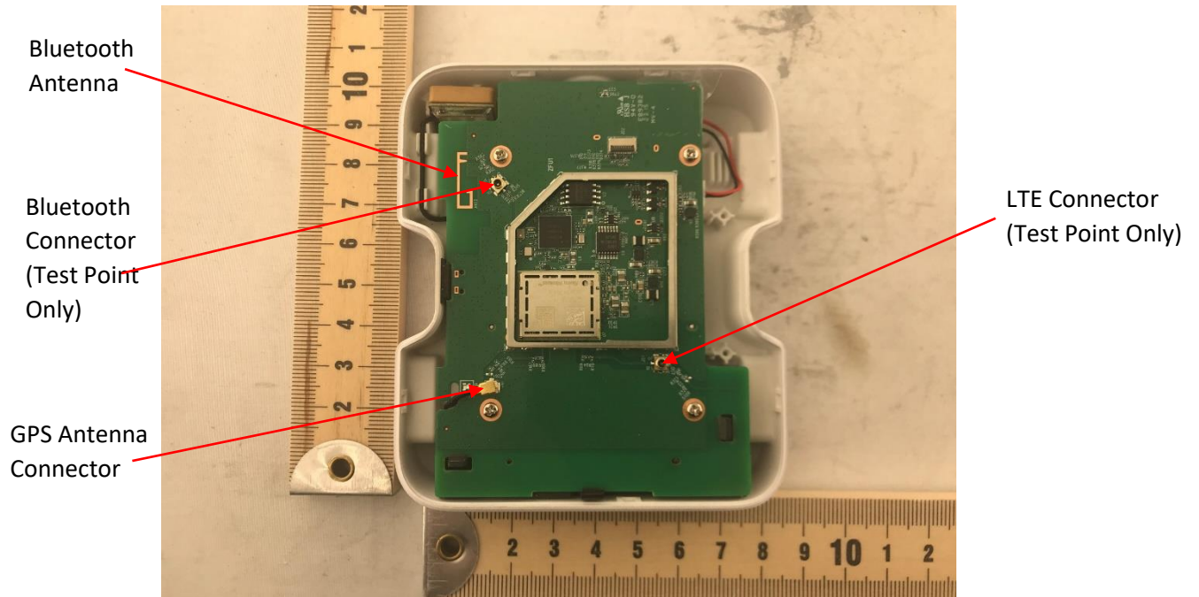
Photograph 3: Internal View of DUT With Can Off
