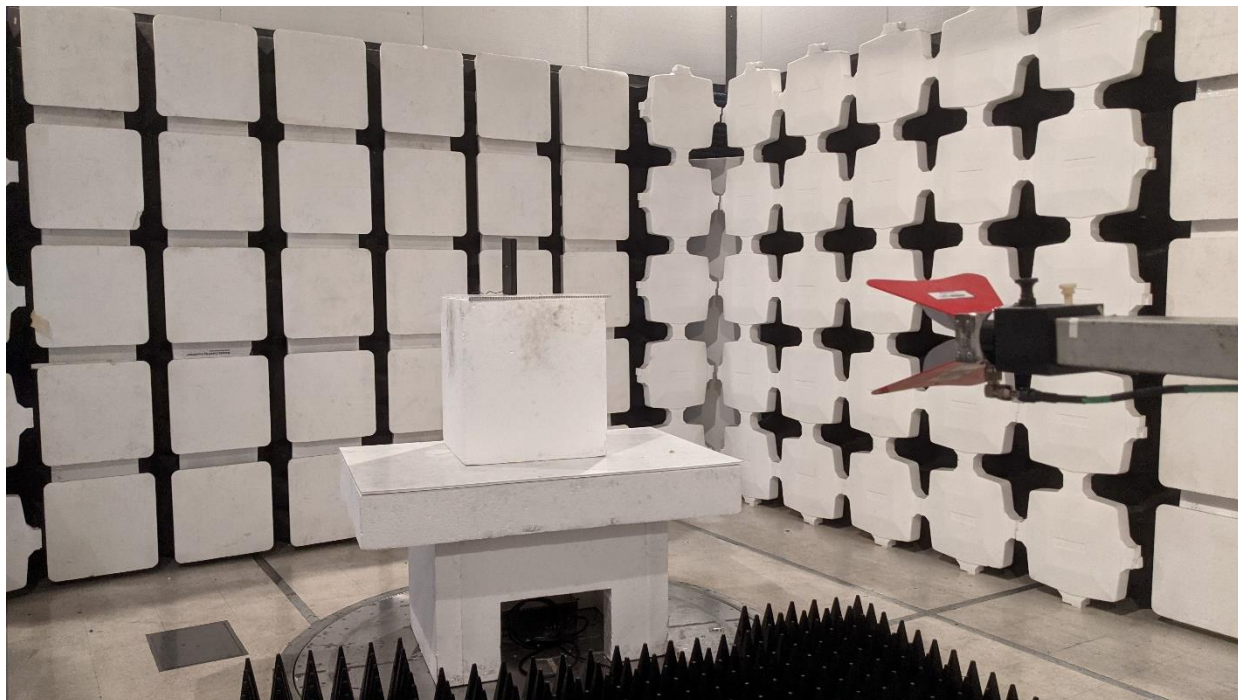
Radiated Emissions
