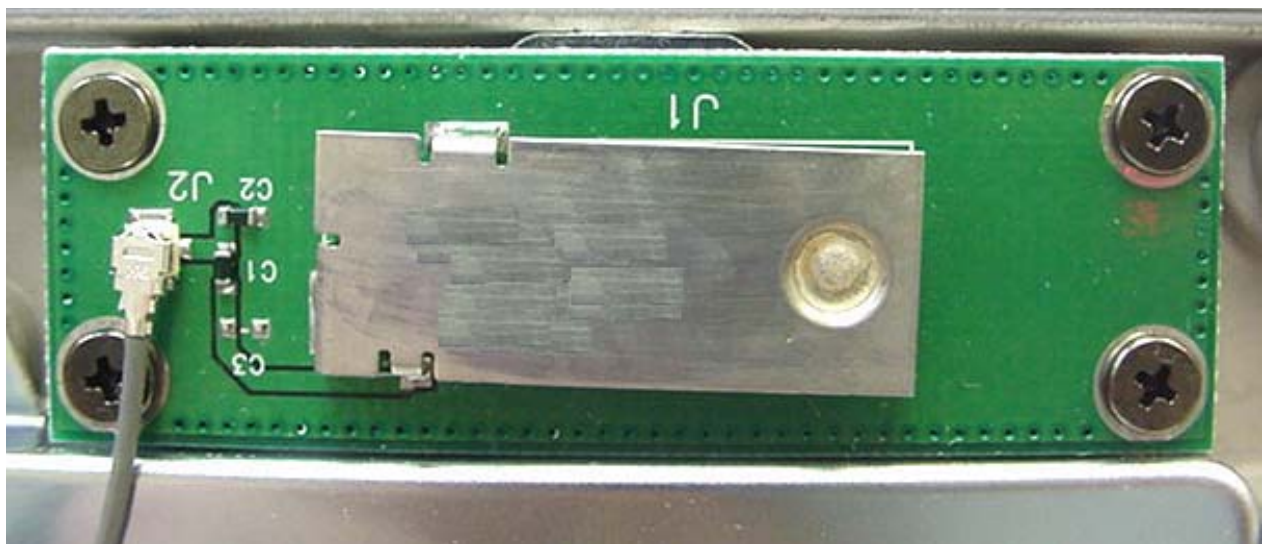
Internal RangeStar Surface-Mount Antenna
