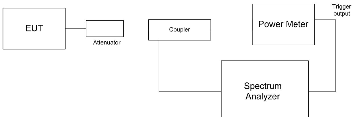
Figure 7.2.1 Peak-to-average power test setup
