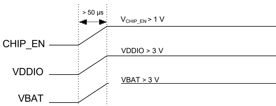
Figure 4: Power-up Timing
