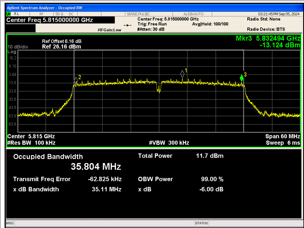
-6dB Bandwidth NVNT ac40 5815MHz Ant2
