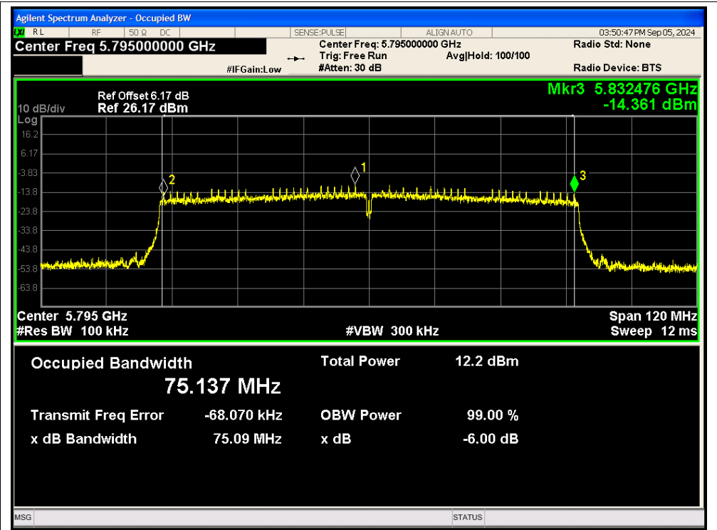
-6dB Bandwidth NVNT ac80 5795MHz Ant2
