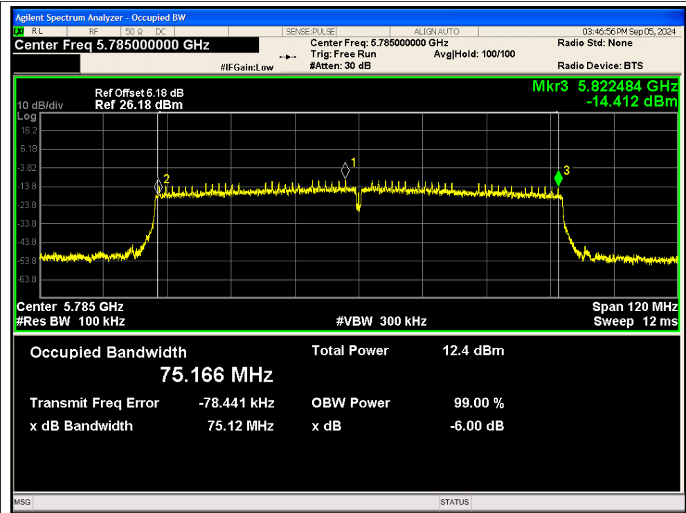
-6dB Bandwidth NVNT ac80 5785MHz Ant2
