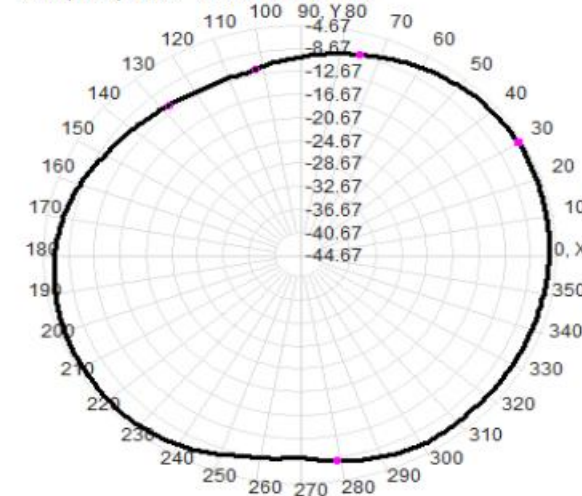
Total(H-XY), Max= -5.50dBi, CirD=6.47
