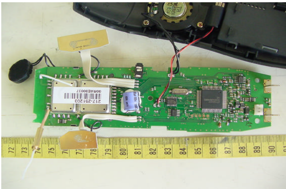
Solder View of Handset's Main PCB
