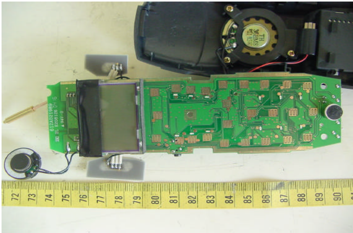
Component View of Handset's Main PCB
