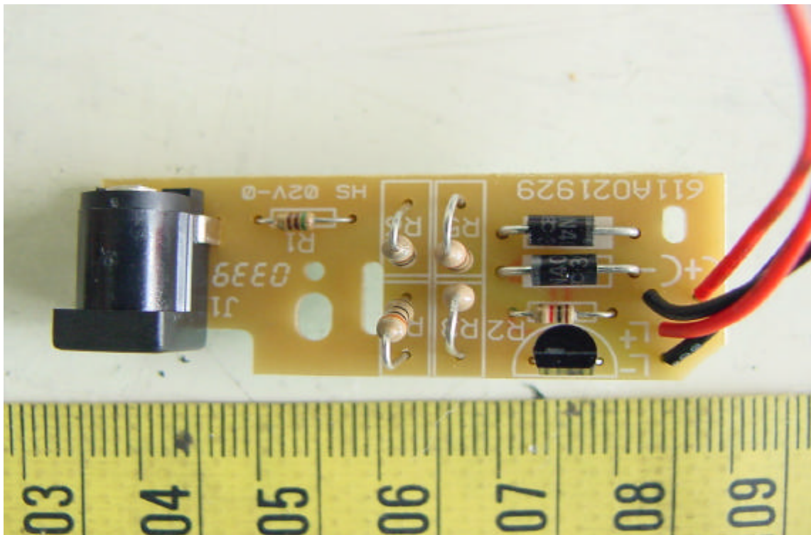
Component View of Charger's Main PCB
