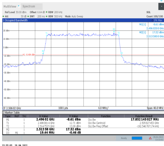
1-N41--30-20-L-1-DFT-QPSK-Outer_Full-50@0-Ant0 -17.852-19.440-≤20-PASS
