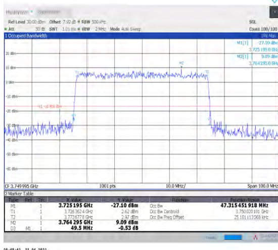
1-N78-3700-3800--30-50-M-9-CP-256QAM-Outer_Full-133@0-Ant0-47.315-49.500-≤50-PASS
