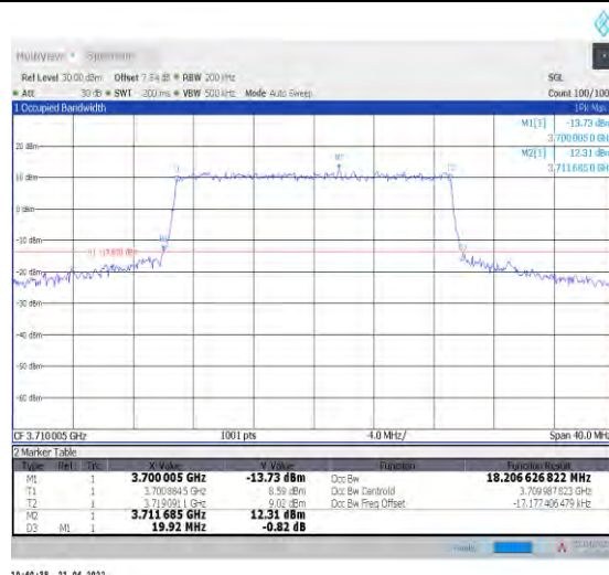
1-N78-3700-3800--30-20-L-6-CP-QPSK-Outer_Full- 51@0-Ant0-18.207-19.920-<20-PASS
