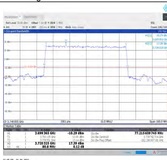
1-N78-3700-3800--30-80-L-2-DFT-PI2BPSK-Outer_ Full-216@0-Ant0-77.216-80.800-≤80-PASS
