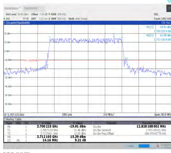
1-N78-3700-3800--30-15-L-1-DFT-QPSK-Outer_Full- 36@0-Ant0-12.828-14.160-≤15-PASS
