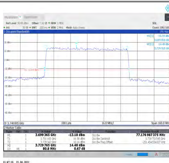
1-N78-3700-3800--30-80-L-4-DFT-64QAM-Outer_Fu ll-216@0-Ant0-77.177-80.800-≤80-PASS
