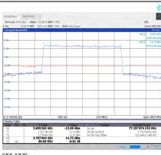
1-N78-3700-3800--30-80-L-3-DFT-16QAM-Outer_Full I-216@0-Ant0-77.297-80.960-≤80-PASS
