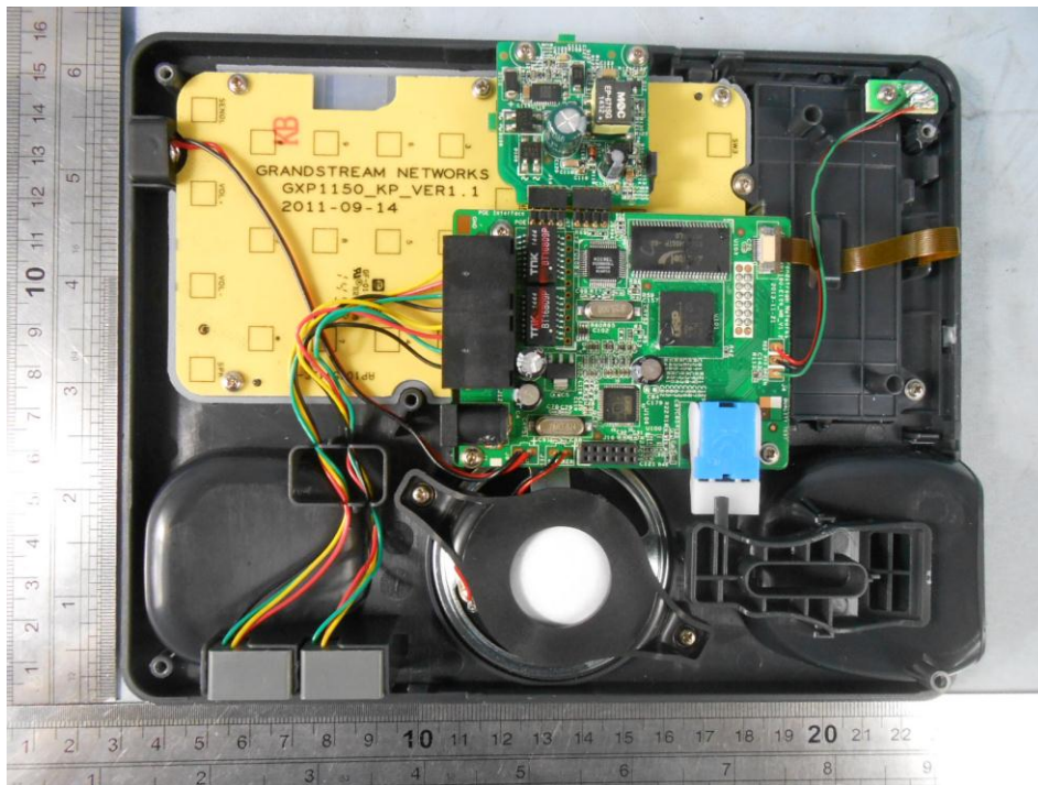
EUT-Uncovered View #2
