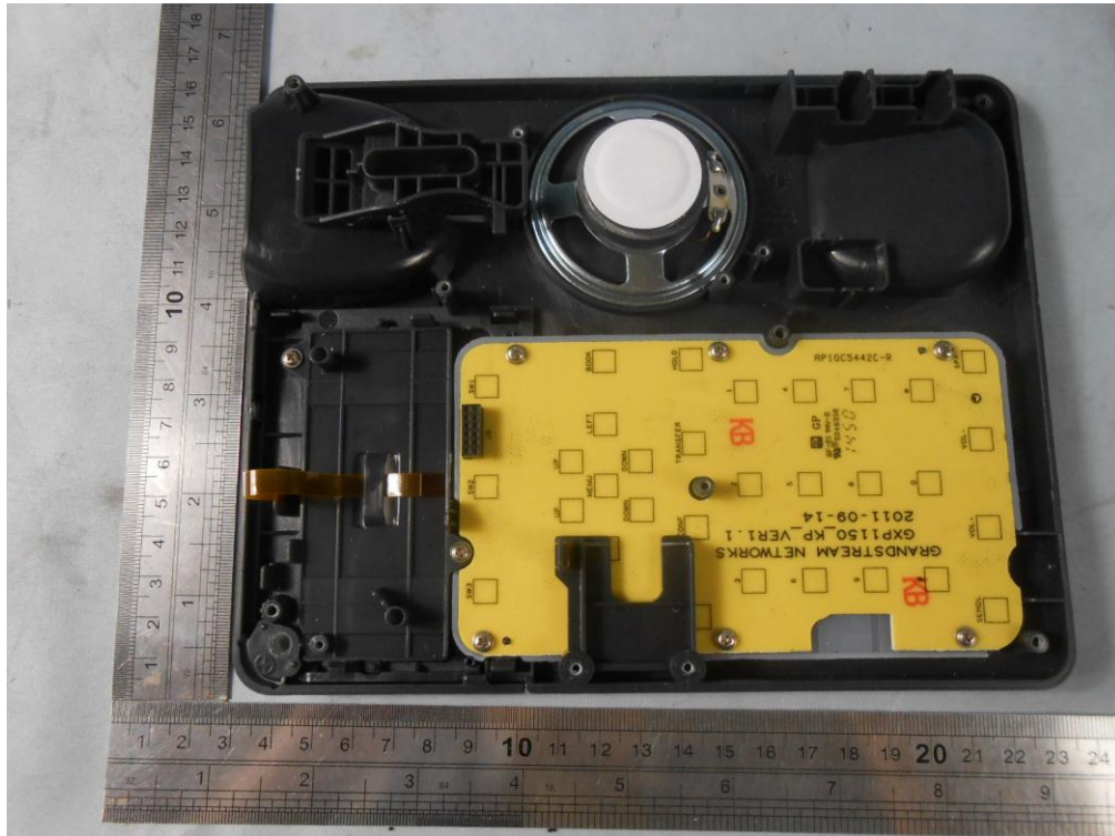
EUT-Uncovered View #3
