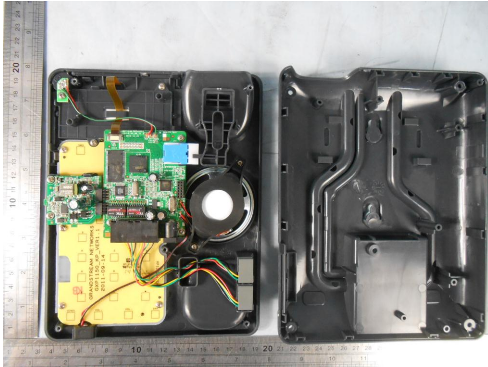
EUT-Uncovered View #1
