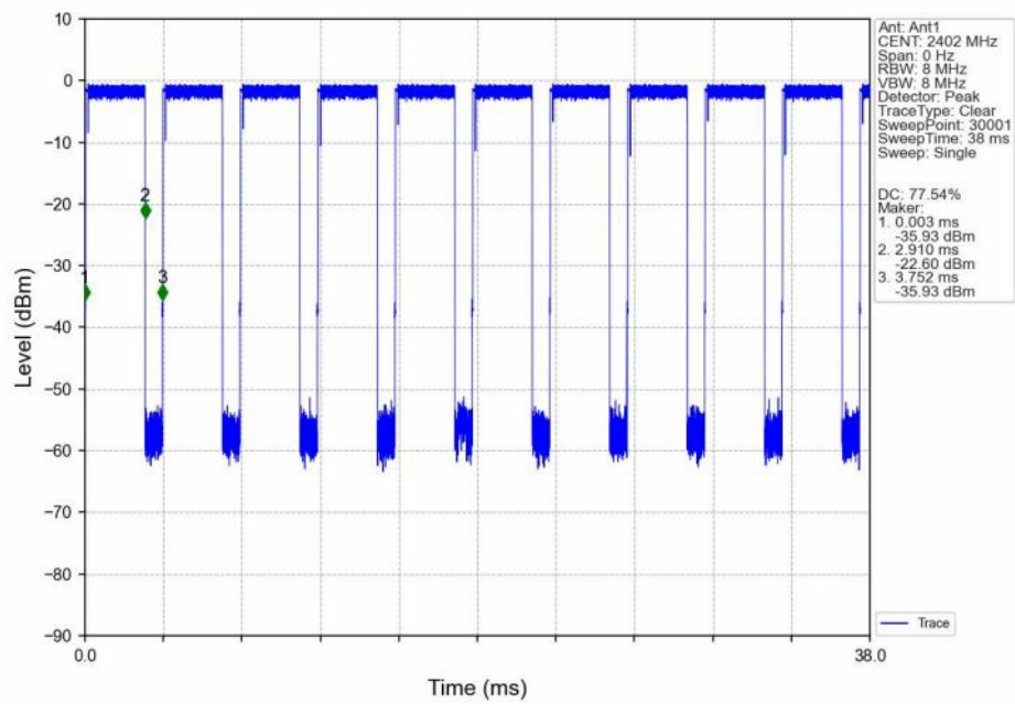
Pi/4DQPSK_2DH5_LCH_2402MHz_Ant1_NTNV
