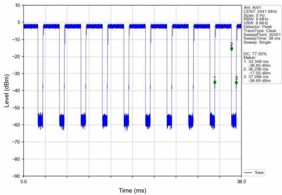
8DPSK_3DH5_MCH_2441MHz_Ant1_NTNV
