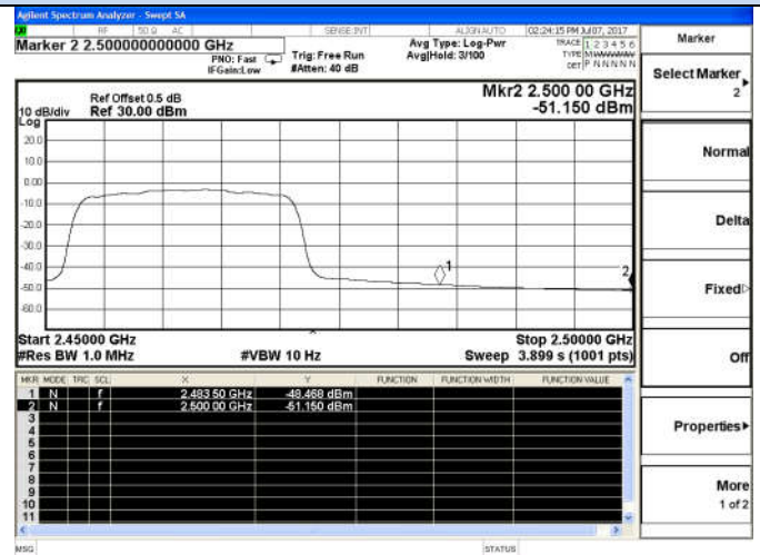
802.11n(HT20)-High channel(Average)
