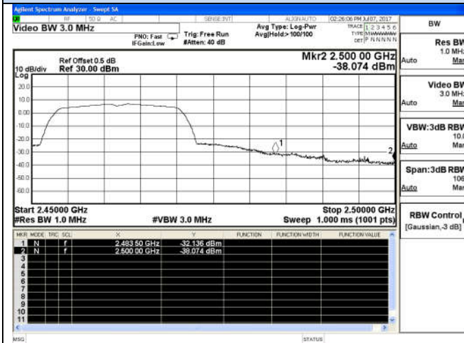
802.11n(HT20)-High channel(Peak)
