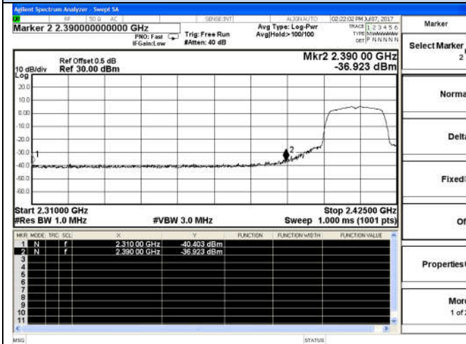
802.11n(HT20)-Low channel(Peak)
