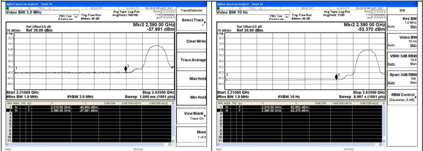
802.11b-Low channel(Peak)
