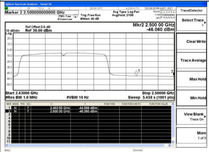
802.11n(HT40)-High channel(Average)
