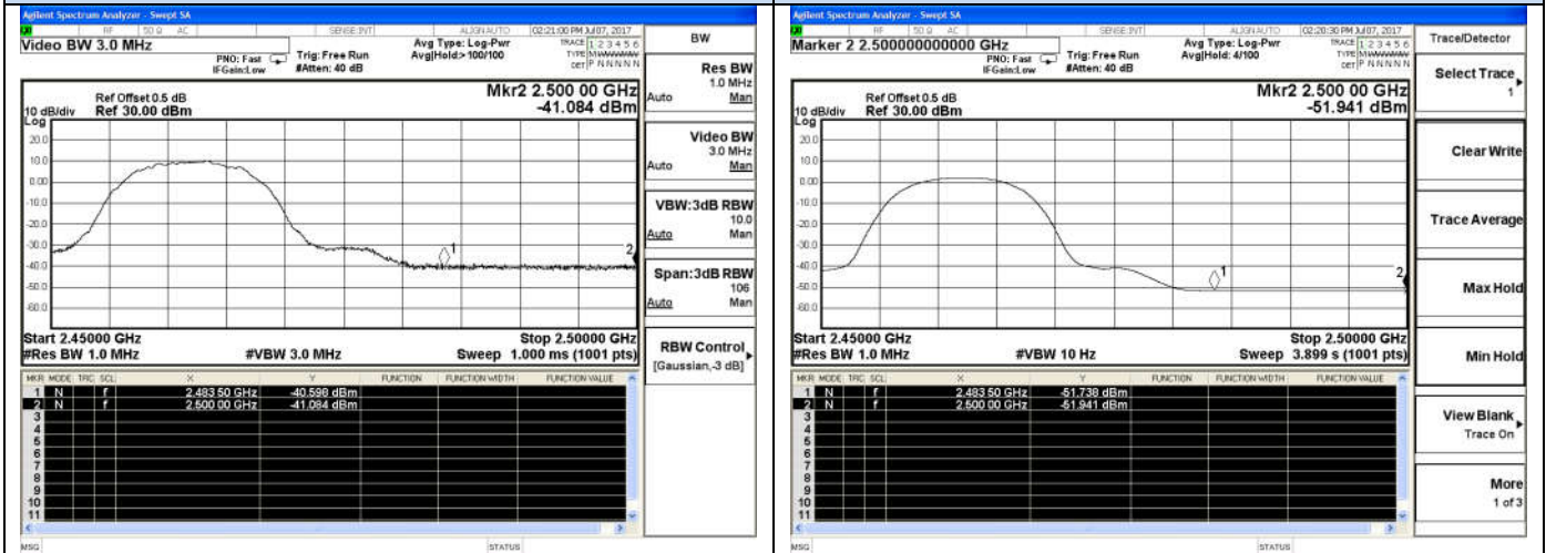
802.11b-High channel(Peak)
