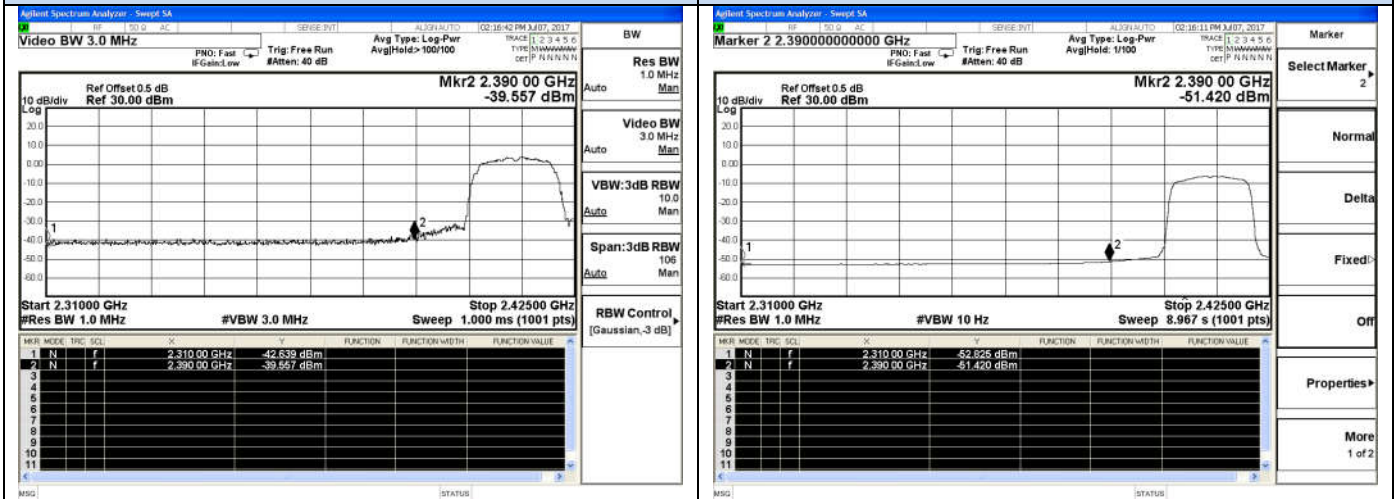
802.11g-Low channel(Peak)
