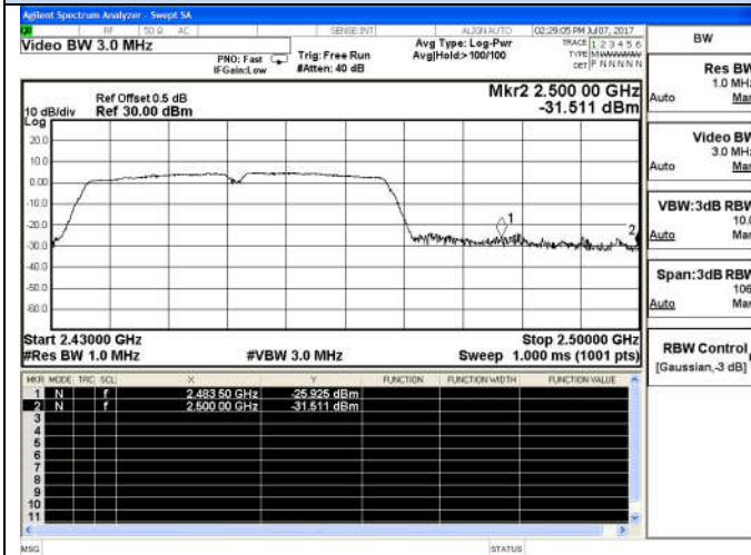
802.11n(HT40)-High channel(Peak)
