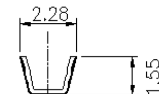
SECTION L-L
