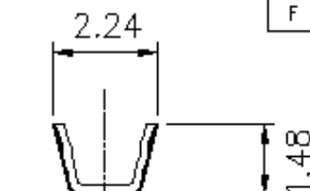
SECTION M-M
